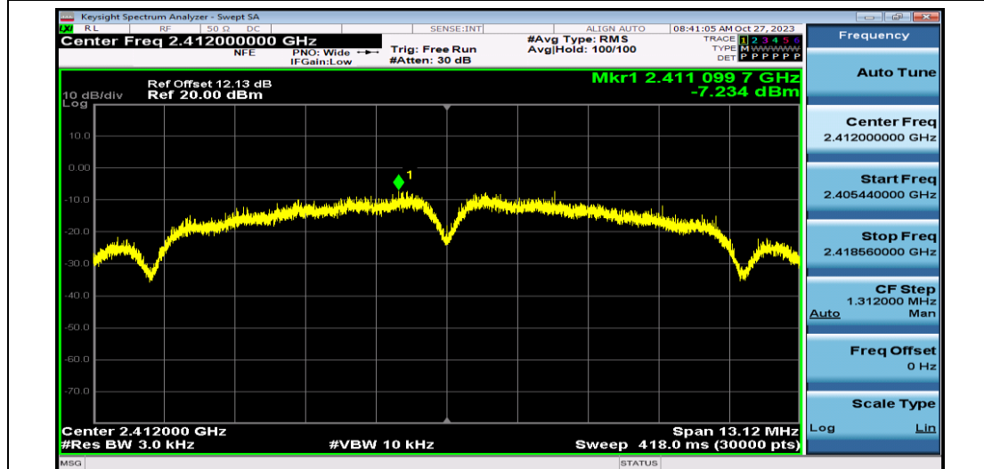
11B-Ant1-2412
