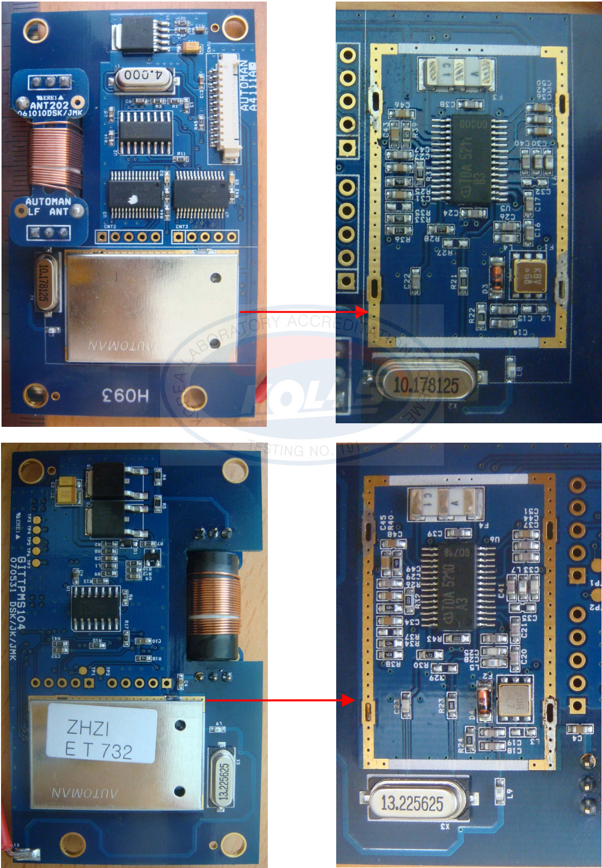
<Photograph 8: RF Board>
