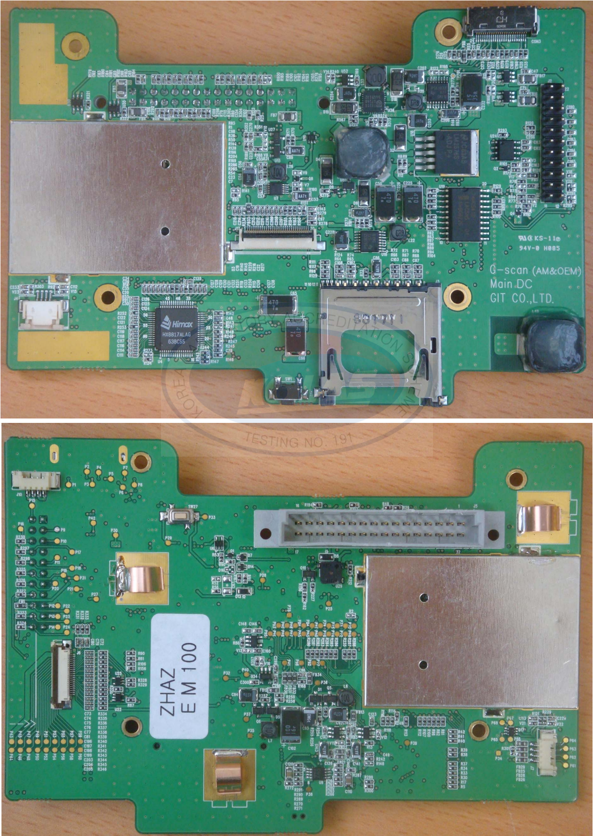
<Photograph 2: Main Board >
