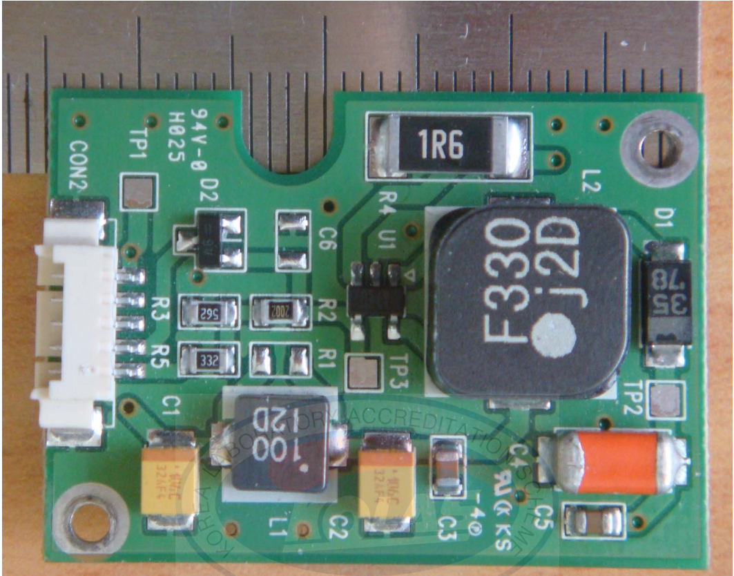
<Photograph 4: LED Backlight Board >
