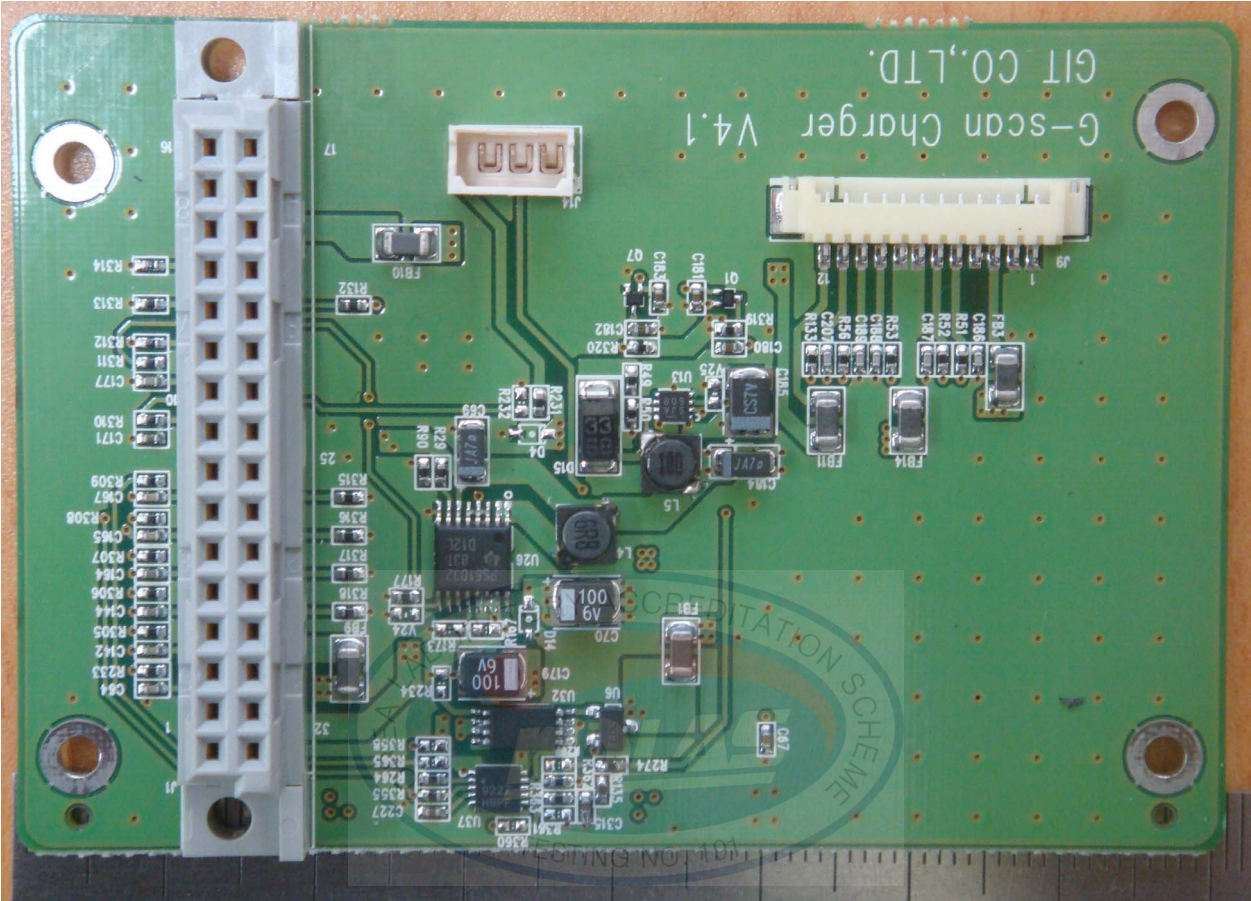
<Photograph 7: Charger Board>
