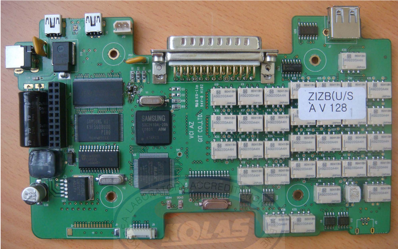
<Photograph 3: VCI Board >
