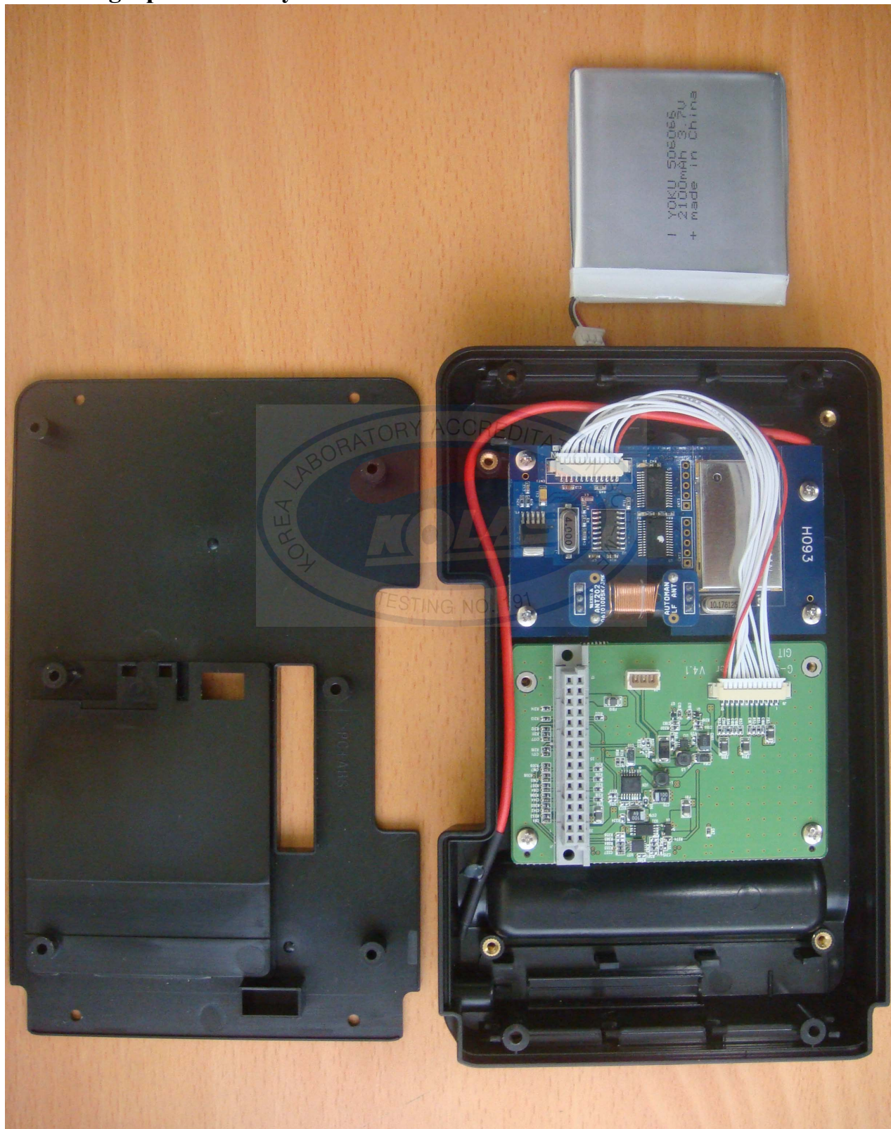
<Photograph 6: Battery Pack Cover removed>
