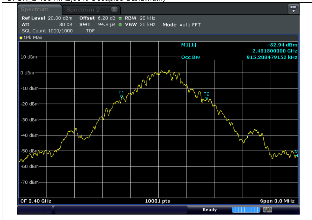
GFSK_2 480 MHz(99% Occupied Bandwidth)
