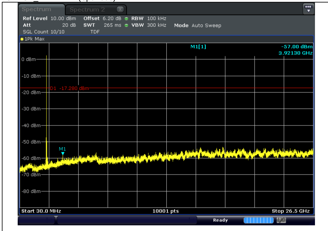
8DPSK_2_441 MHz(Spurious)
