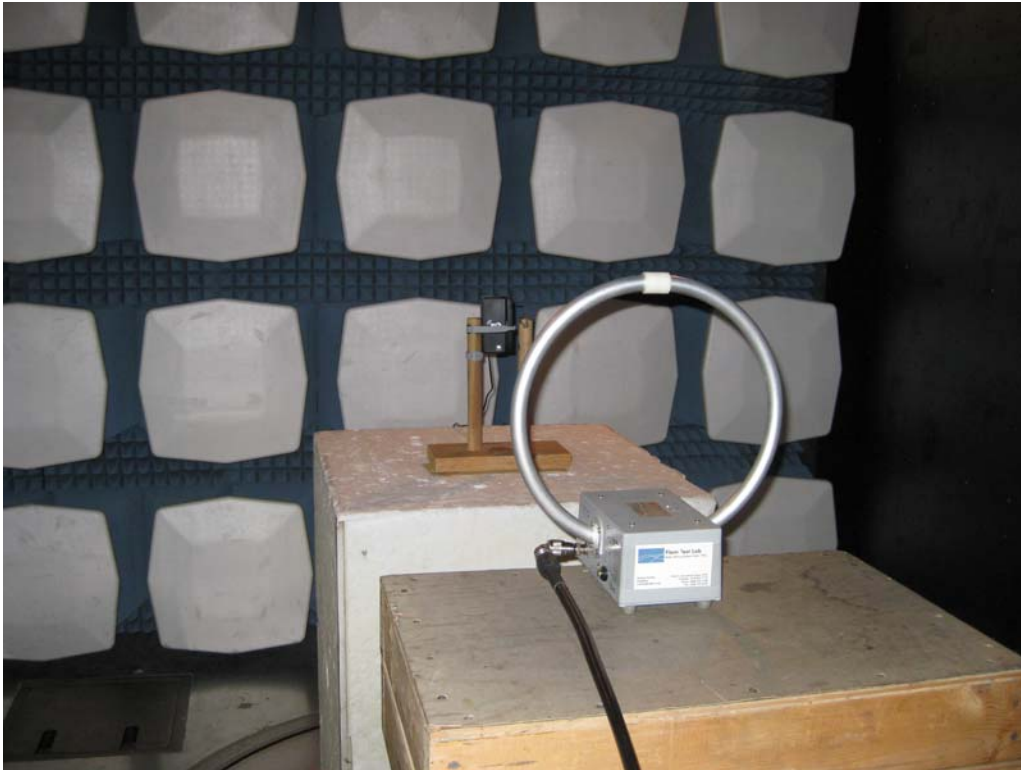
Model 4100 - Radiated
