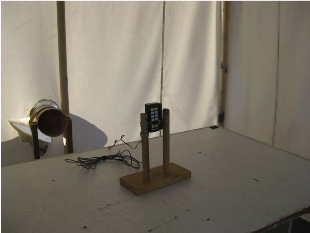
Model 4110: OATS #2
