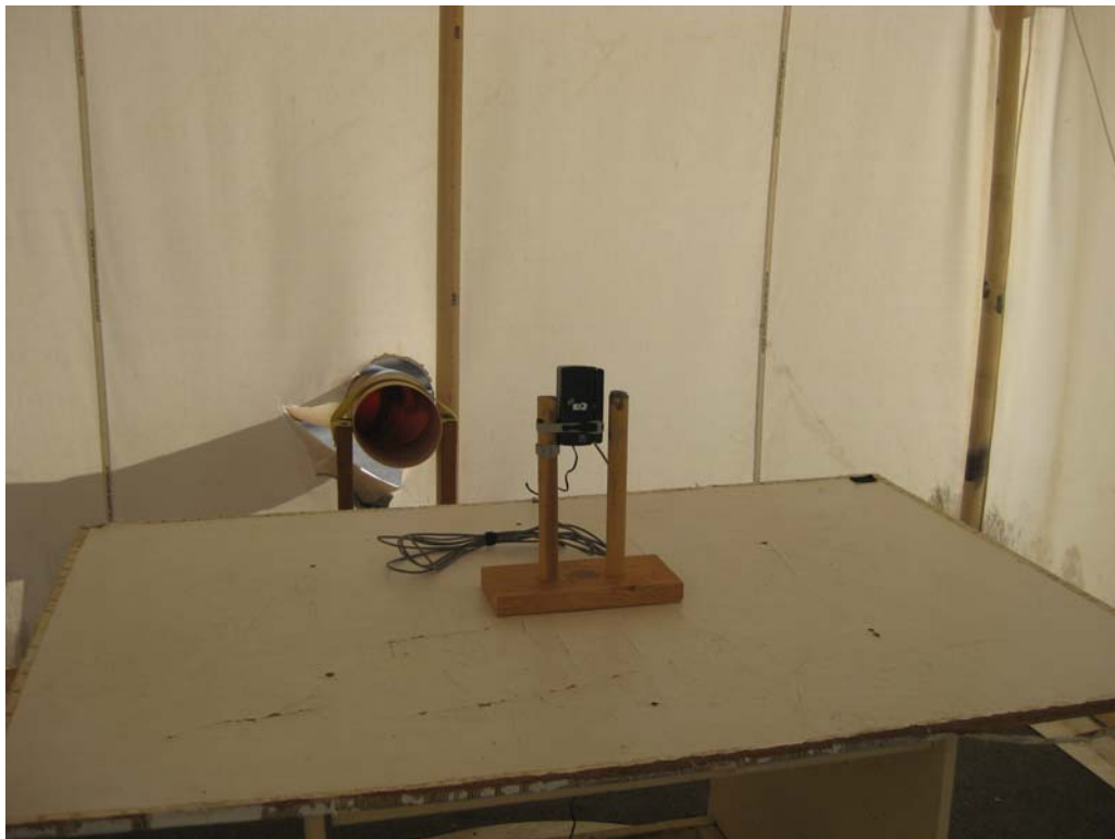
Model 4100 – OATS #2
