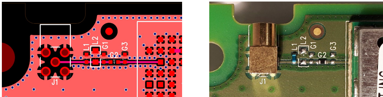
Figure 8 FCC and ISED approved trace design layout and picture for external antennas with MMCX connector
