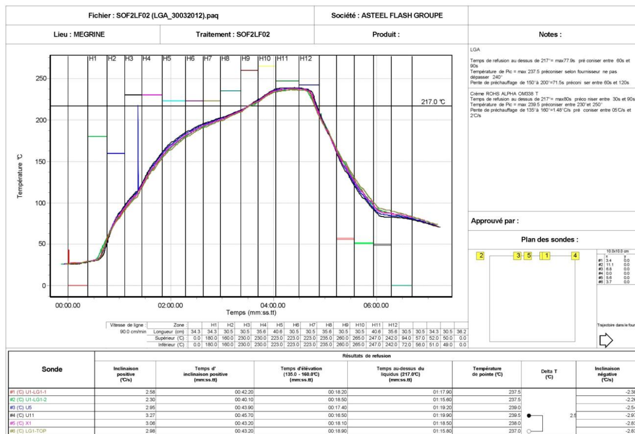
Figure 26: Preliminary OSDI Module Reflow Profile and Set Points.
