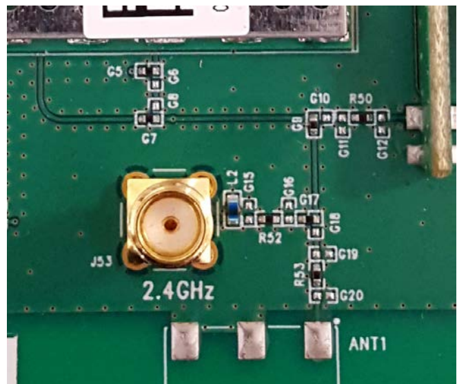
Figure 14 FCC and IC approved trace design layout and picture for the M antenna of section 4.2.1
