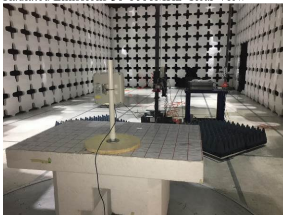
Radiated Emissions Above 1GHz - Rear View
