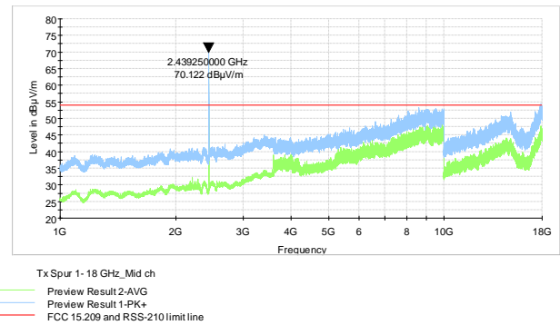
Figure 7.7-14: Radiated spurious emissions on Mid
