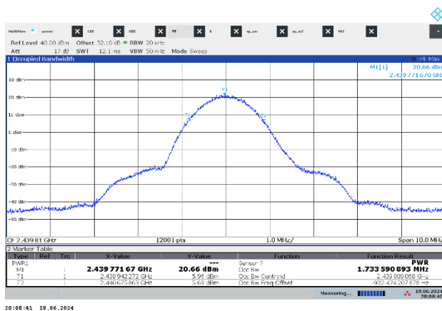
Figure 7.5-5: 99% occupied bandwidth on Mid Channel
