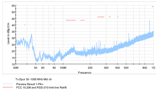
Figure 7.7-13: Radiated spurious emissions on Mid
