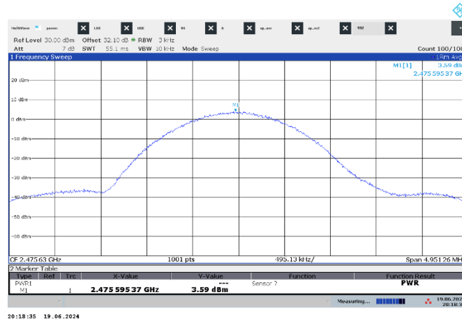
Figure 7.8-3: PSD on high channel
