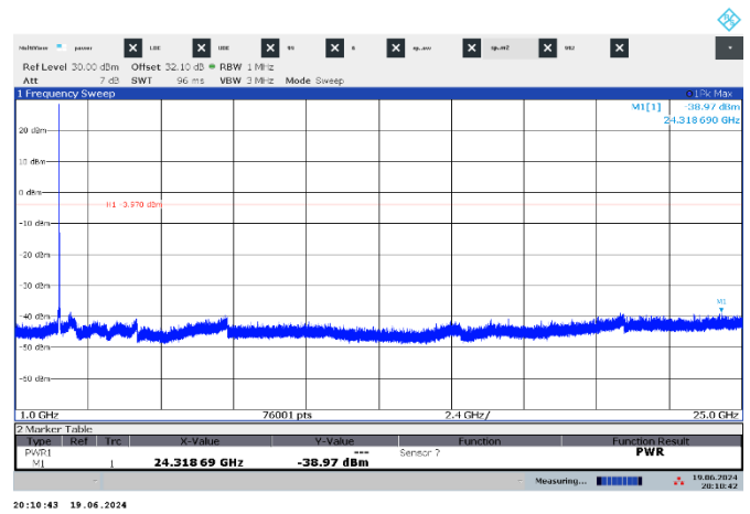
Figure 7.7-8: Conducted spurious emissions on Mid Channel 1-25 GHz
