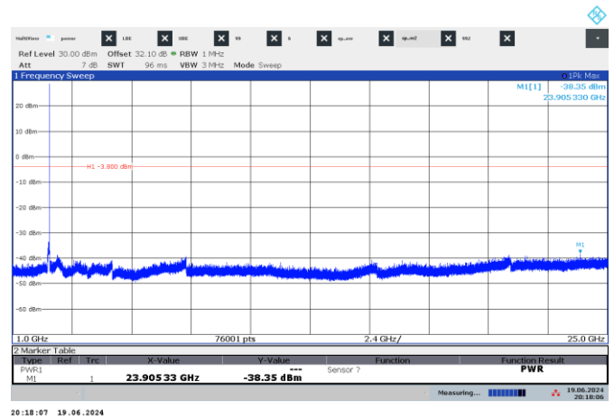
Figure 7.7-10: Conducted spurious emissions on High Channel 1-25 GHz
