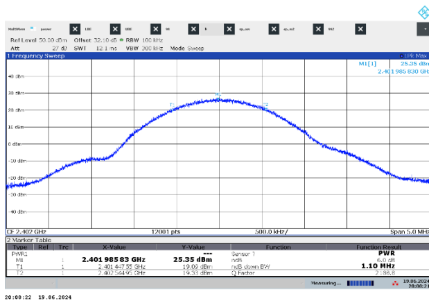
Figure 7.5-1: 6 dB bandwidth on Low Channel
