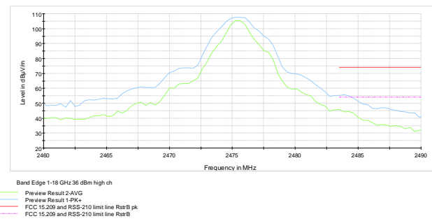
Figure 7.7-2: Radiated Band edge spurious emissions at 2483.5 MHz
