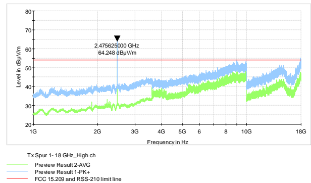
Figure 7.7-16: Radiated spurious emissions on High
