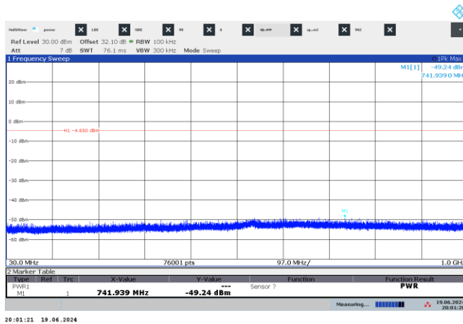
Figure 7.7-5: Conducted spurious emissions on Low Channel 30-1000 MHz
