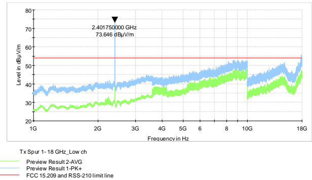
Figure 7.7-12: Radiated spurious emissions on Low
