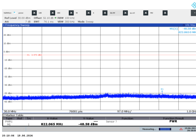
Figure 7.7-7: Conducted spurious emissions on Mid Channel 30-1000 MHz
