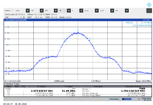
Figure 7.5-6: 99% occupied bandwidth on High Channel
