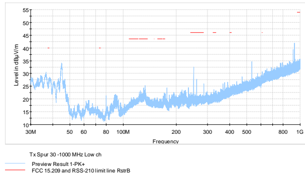
Figure 7.7-11: Radiated spurious emissions on Low
