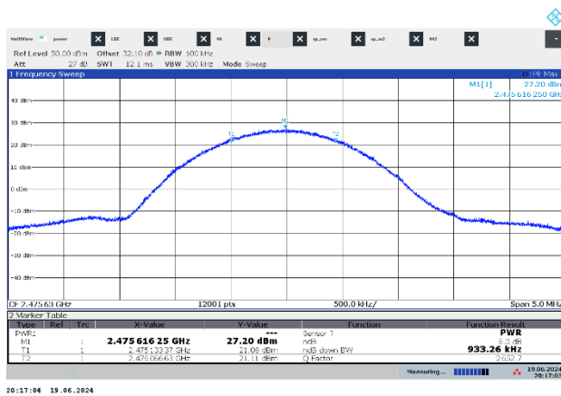
Figure 7.5-3: 6 dB bandwidth on High Channel
