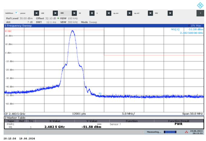
Figure 7.7-4: Band edge spurious emissions at 2483.5 MHz (Conducted)
