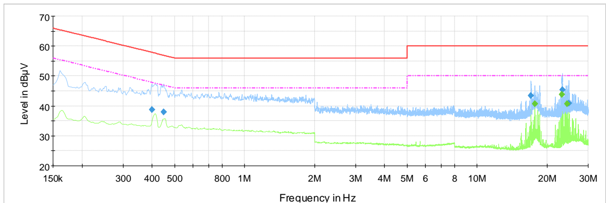
Plot 7.4-1: Conducted emissions on phase line
