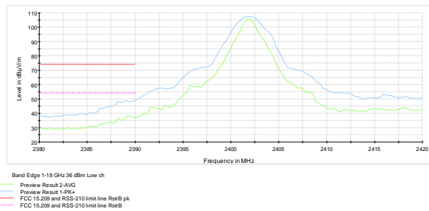
Figure 7.7-1: Radiated Band edge spurious emissions at 2400 MHz
