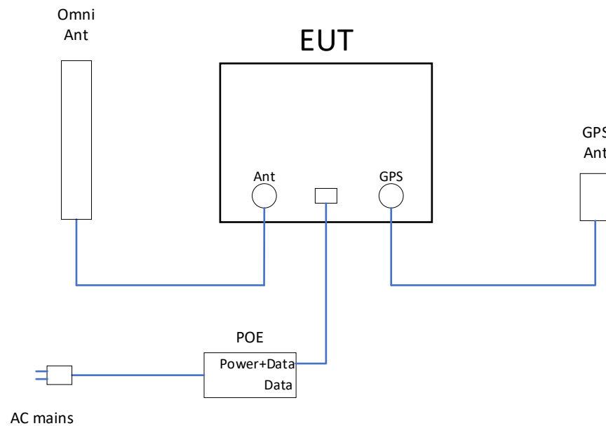
Figure 4.5-1: block diagram
