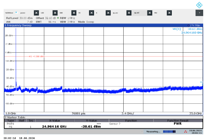
Figure 7.7-6: Conducted spurious emissions on Low Channel 1-25 GHz
