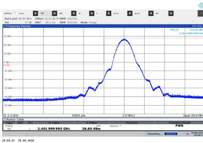
Figure 7.7-3: Band edge spurious emissions at 2400 MHz (Conducted)
