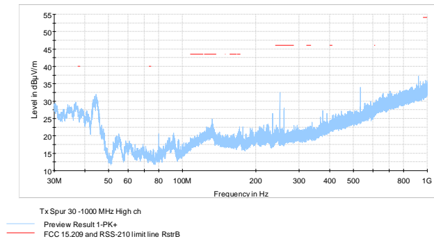
Figure 7.7-15: Radiated spurious emissions on High
