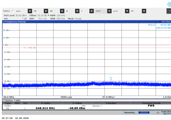
Figure 7.7-9: Conducted spurious emissions on High Channel 30-1000 MHz
