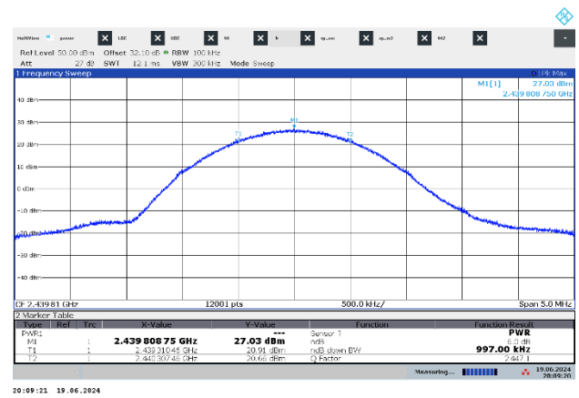
Figure 7.5-2: 6 dB bandwidth on Mid Channel
