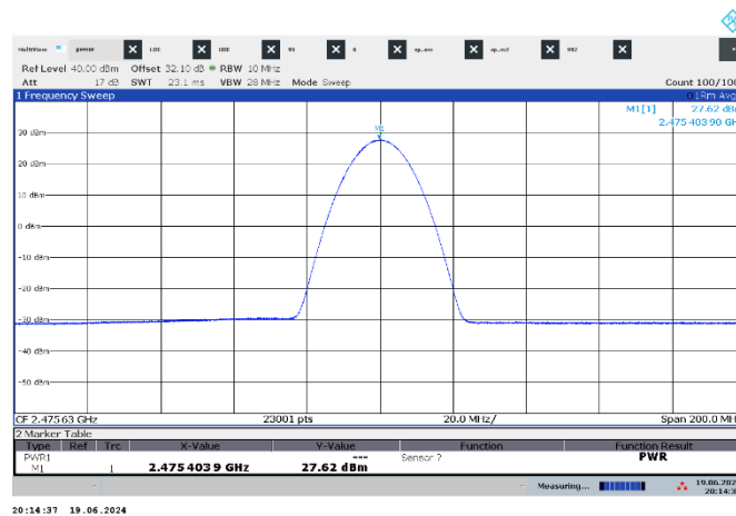
Figure 7.6-3: Output power on high channel
