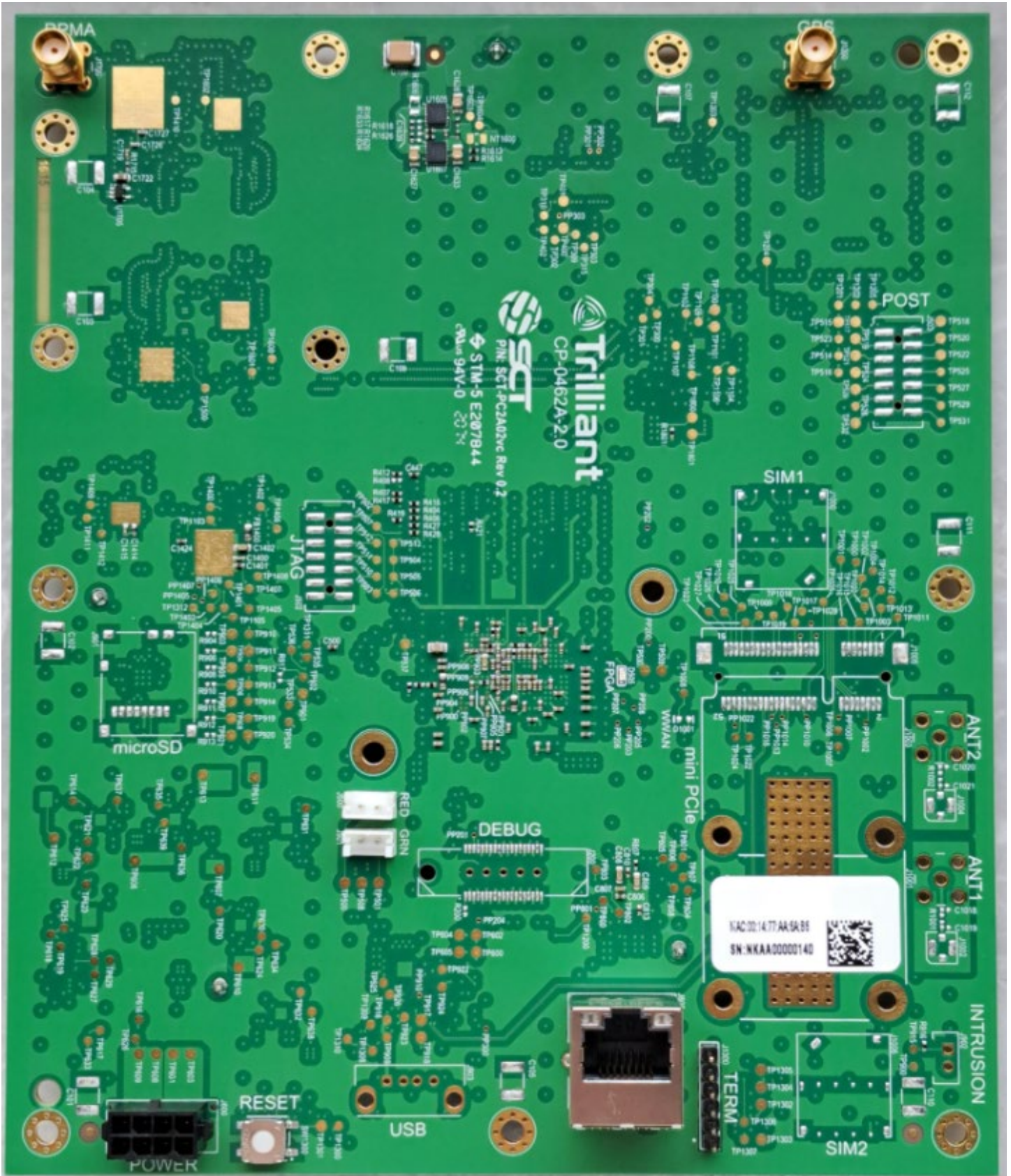
Pliny board top view
