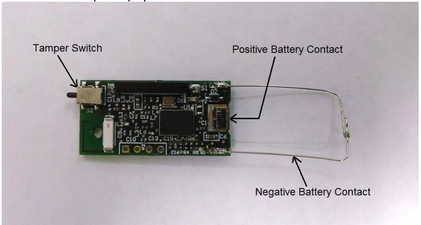
ELK-6023 Transceiver (PCA191) Top View:
