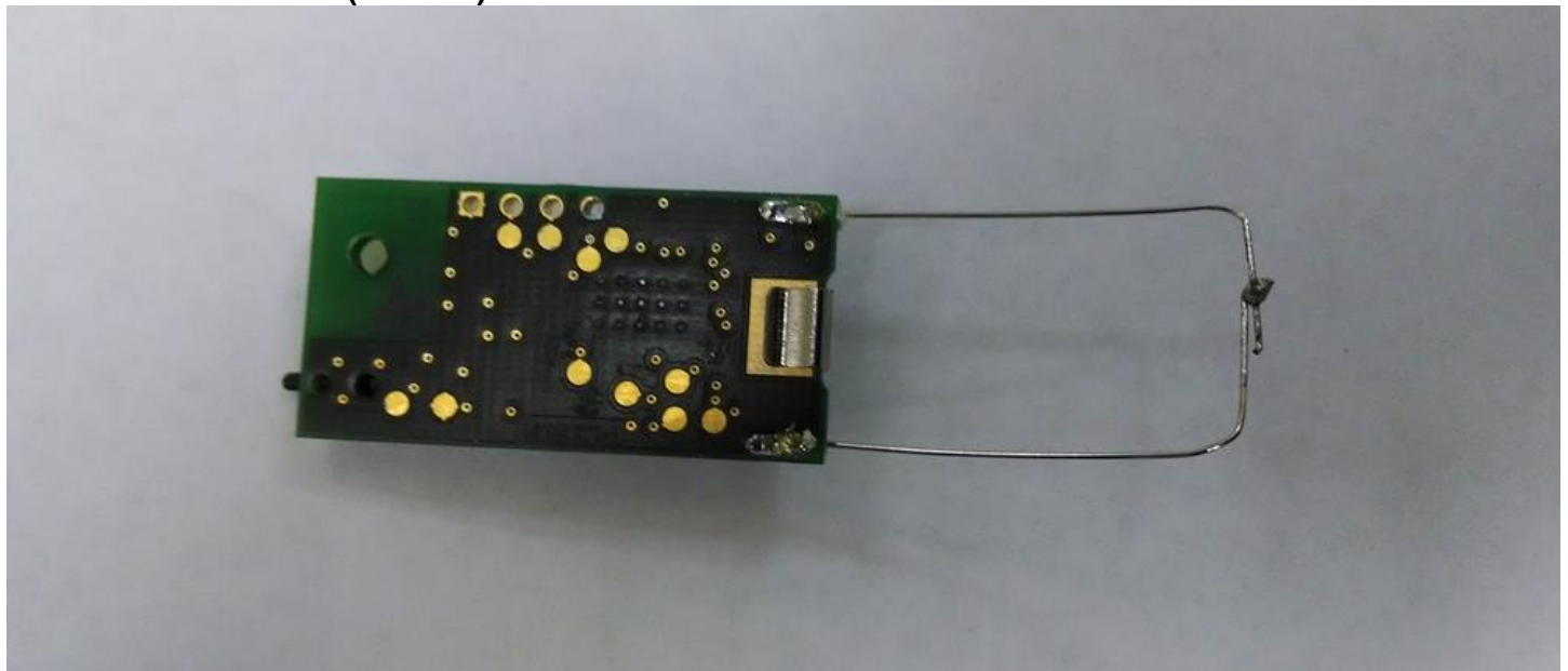
ELK-6023 Transceiver (PCA191) Bottom View:
