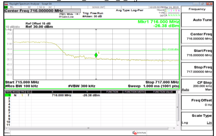
Band12_10MHz_QPSK_50_0_HighCH23130-711
