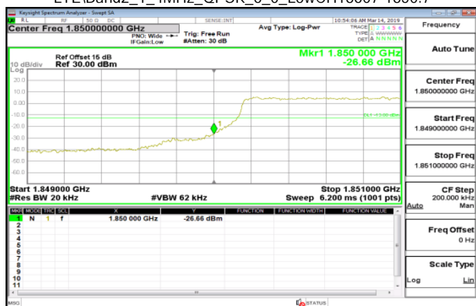
LTE\Band2_1_4MHz_QPSK_6_0_LowCH18607-1850.7
