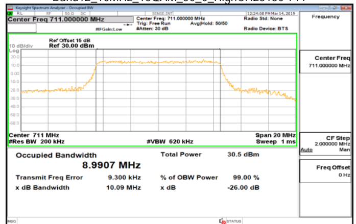
Band12_10MHz_16QAM_50_0_HighCH23130-711
