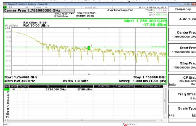
LTE\Band4_20MHz_QPSK_1_99_HighCH20300-1745
