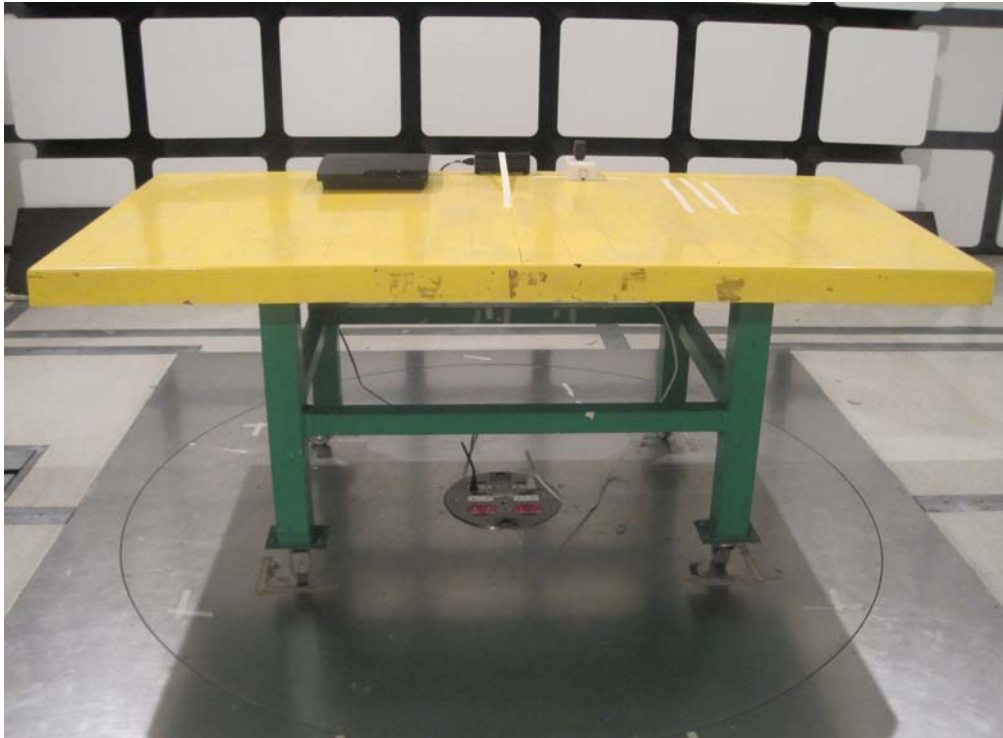
Radiated Emissions below 1GHz
