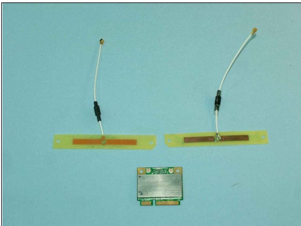
Antenna 2 Model No.: ADP6P-700003
