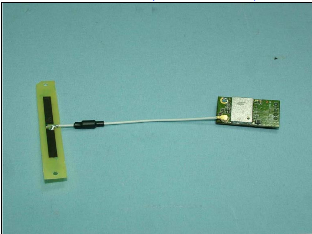
Antenna 2: Printed (Model: ADP6P-70003)
