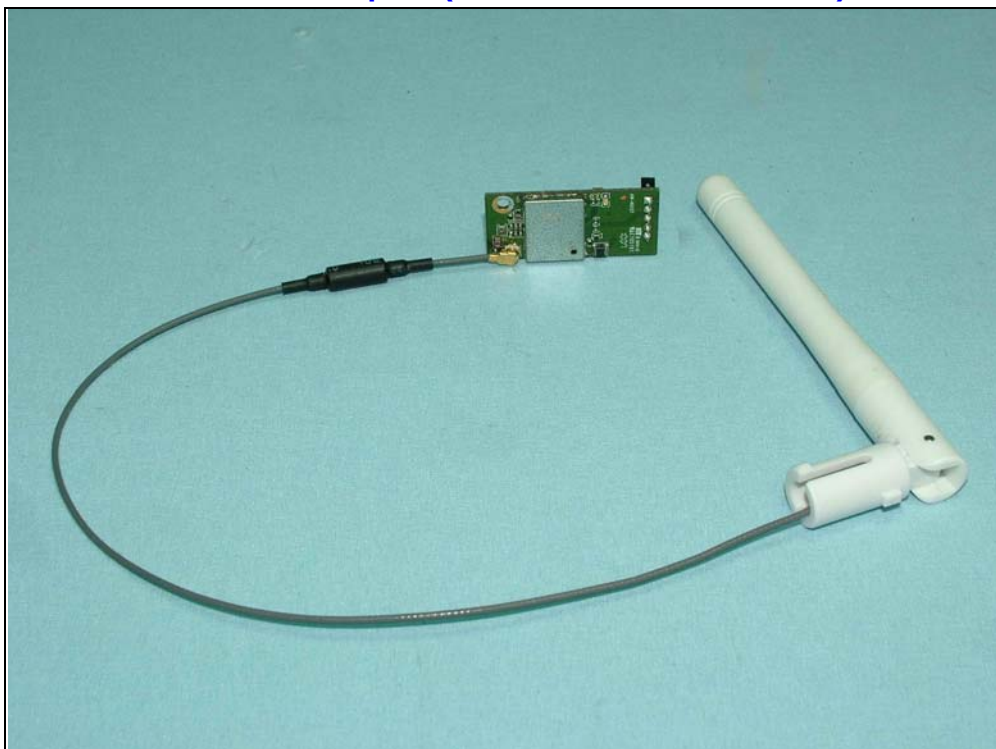
Antenna 1: Dipole (Model: CAR-ATR-179-008)
