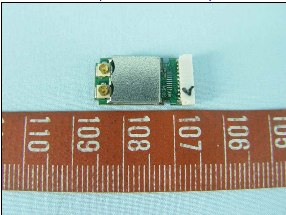
EUT (Two antenna connectors)
