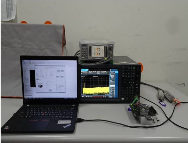
FCC_15_247_902~928MHz_OFDM_Conducted_4.3V_Setup
