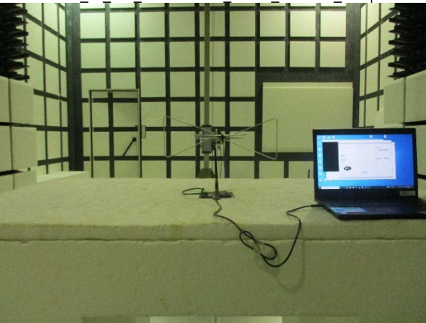
FCC 15 247 902~928MHz OFDM Radiated Setup
