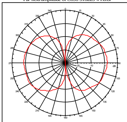
Far-field amplitude of C056-510223-4-H.nsi
