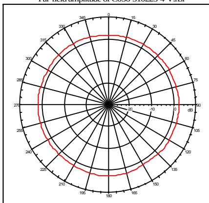
Far-field amplitude of C056-510223-4-V.nsi
