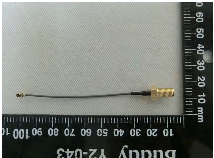
Antenna cable (For Ant. 6 and Ant .7 use)
