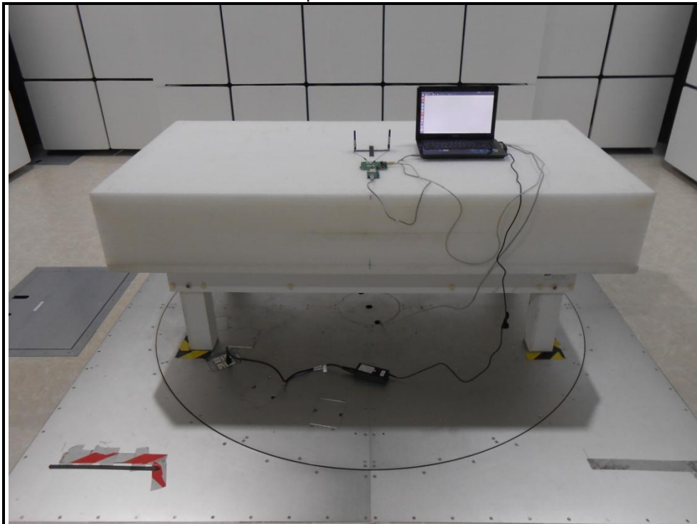
Dipole Antenna
