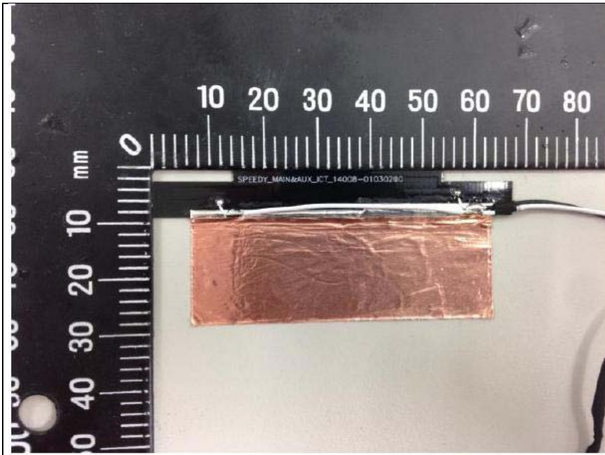
Antenna (Brand: LUXSHARE ICT ; Model : Speedy<Main>)
