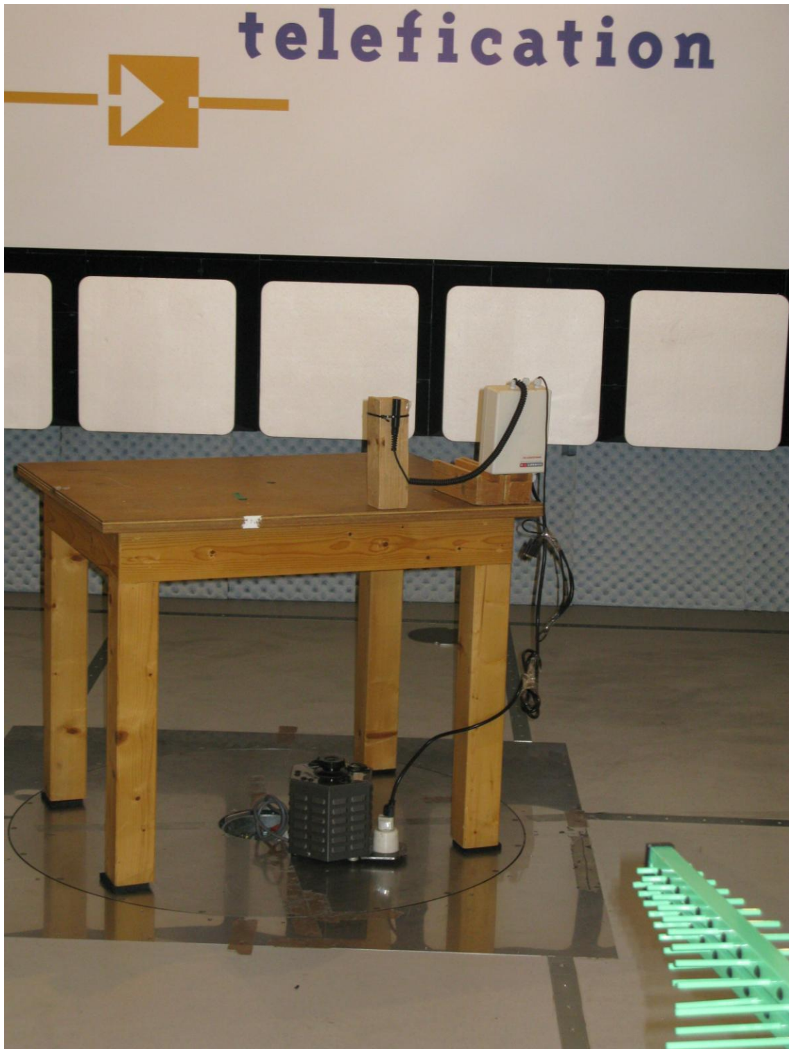
Photograph 4: Test set up 0.03 - 1 GHz (ANT613)
