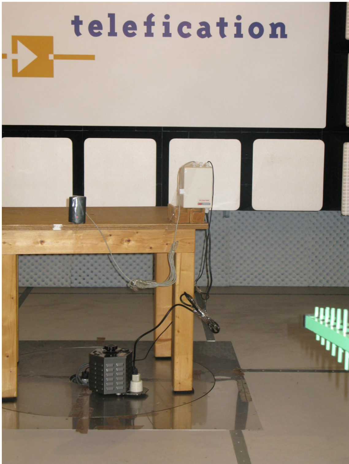
Photograph 6: Test set up 0.03 - 1 GHz (ANT 614)
