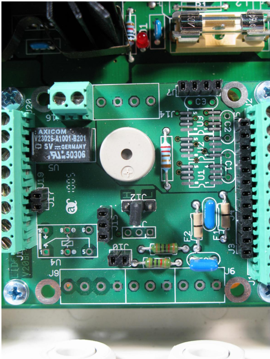
Photograph 4: view on connector board
