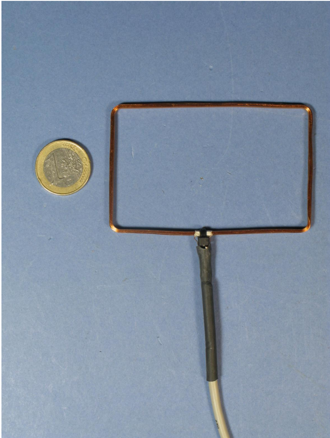
Photograph 4: external antenna type ANT614OEM
