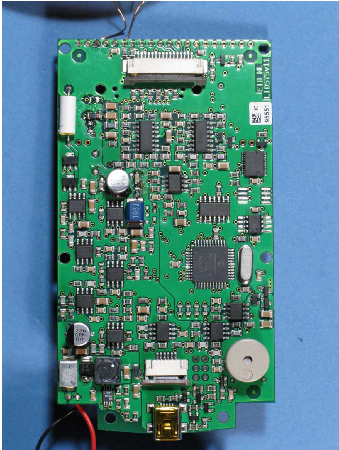
Photograph 3: LID565/575, PCB, component view
