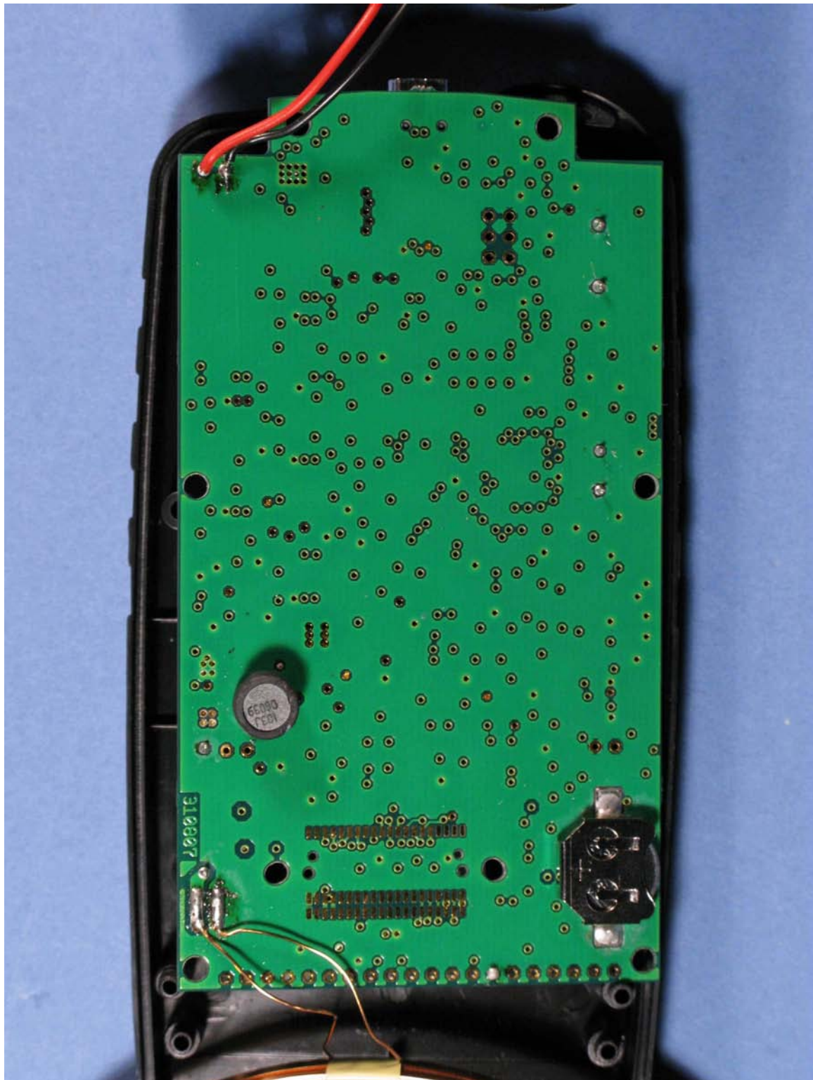
Photograph 4: LID565/575, PCB, copper side
