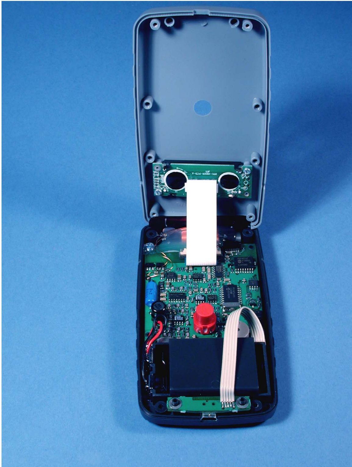
Photograph 1: LID571-x exploded view
