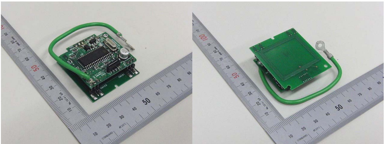
Figure 2 TOP and BOTTOM VIEW OF RFID Reader/Writer Module
