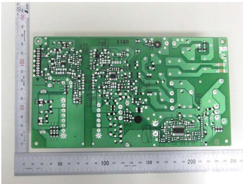
Figure 8 BOTTOM VIEW OF POWER SUPPLY UNIT
