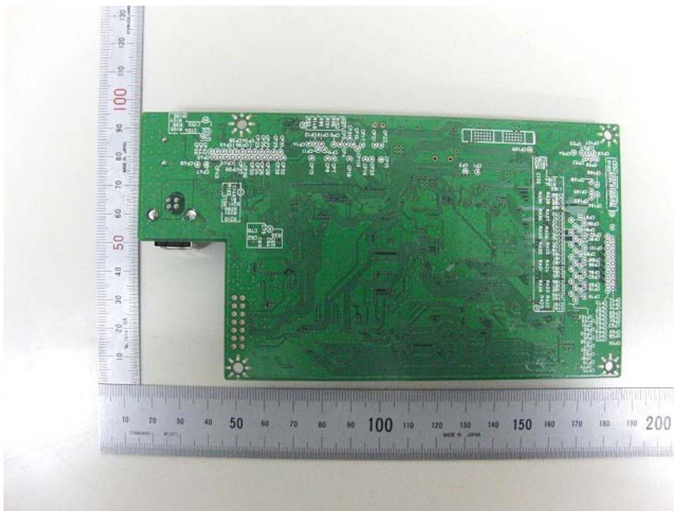
Figure 6 BOTTOM VIEW OF Main BORAD
