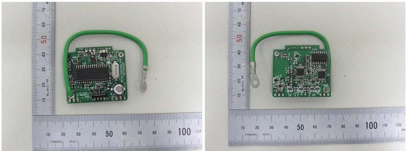
Figure 4 TOP and BOTTOM VIEW OF RFID Reader/Writer Module CONTROL BORAD
