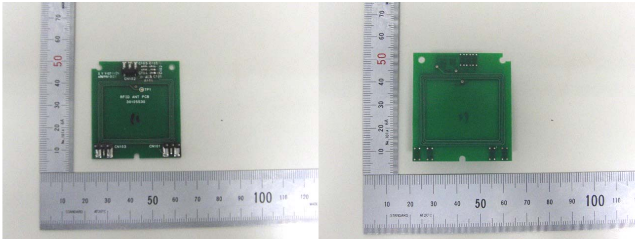
Figure 3 TOP and BOTTOM VIEW OF RFID Reader/Writer Module ANT BORAD
