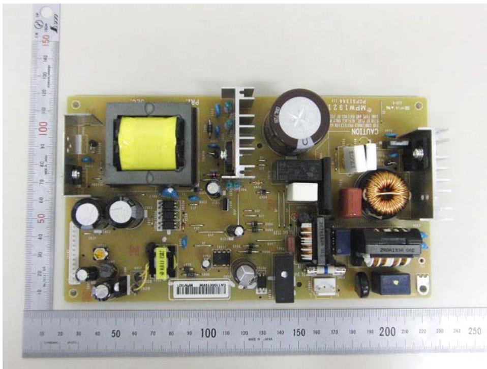
Figure 7 TOP VIEW OF POWER SUPPLY UNIT
