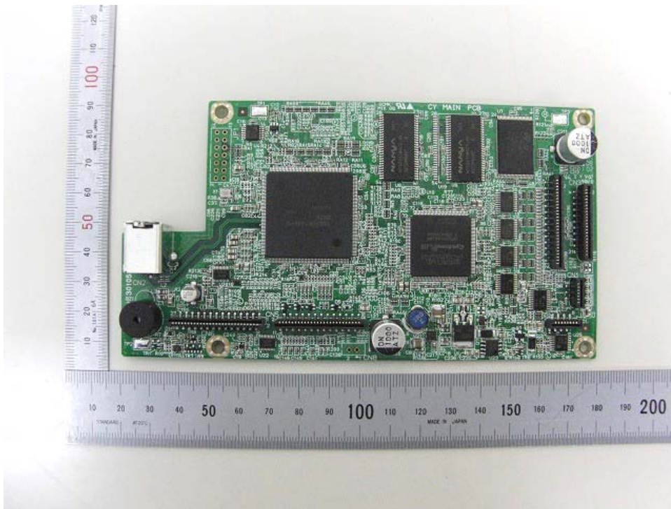
Figure 5 TOP VIEW OF Main BORAD
