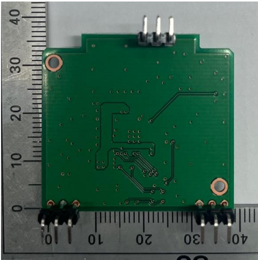
Control PCB
