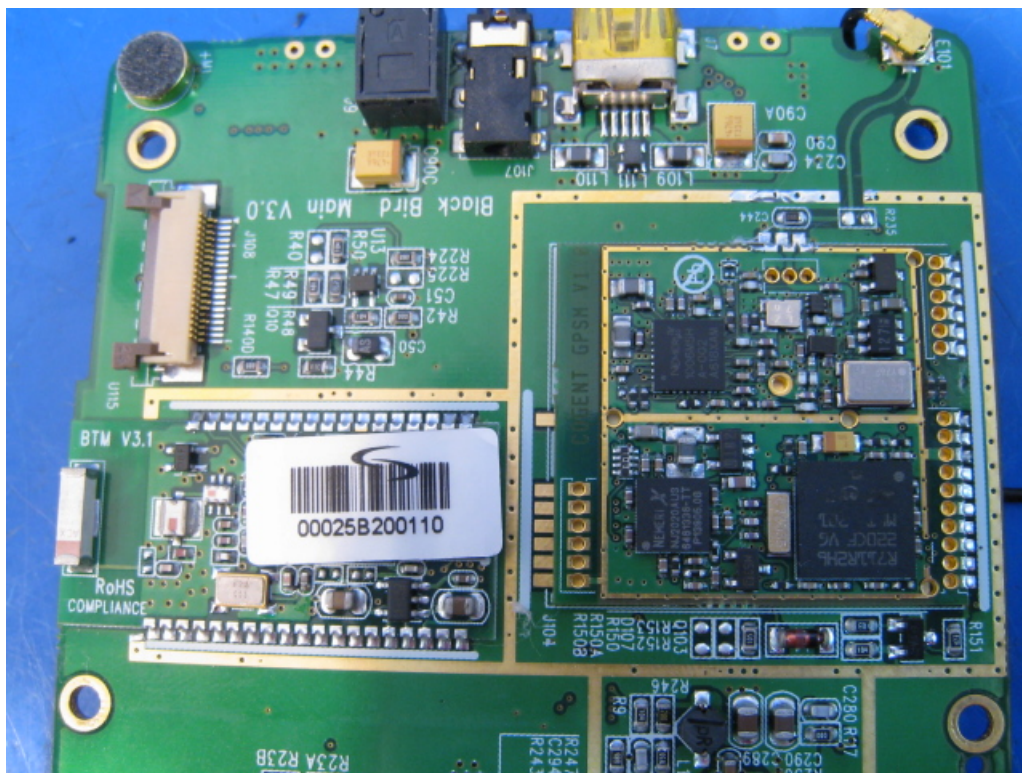
Photo 6 Inside of EUT (GPS module)
