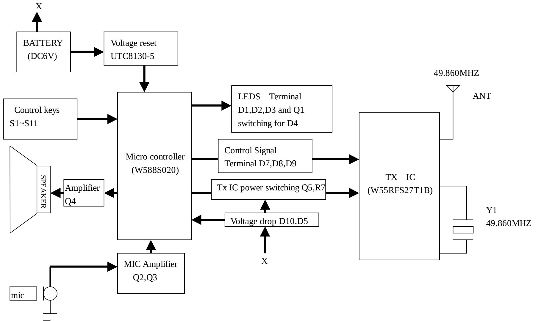
Y3094 Transmitter block diagram (TX)
