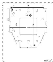
Drilling template
