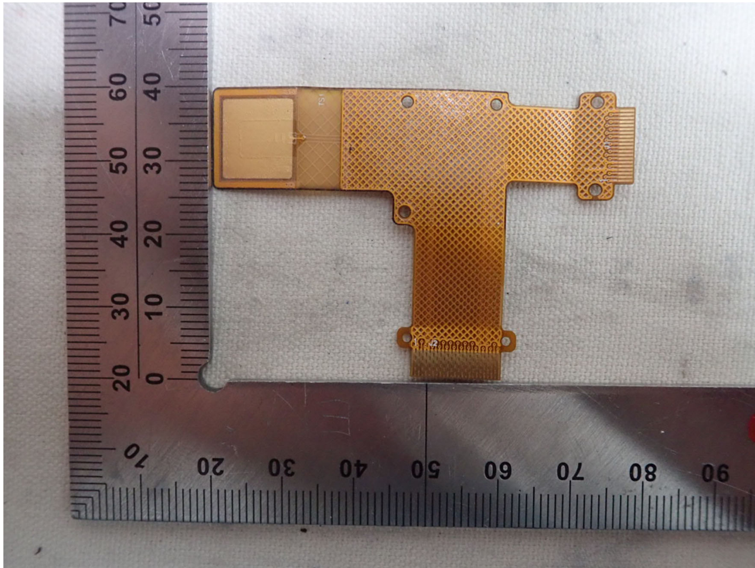
Sensor Film Rear
