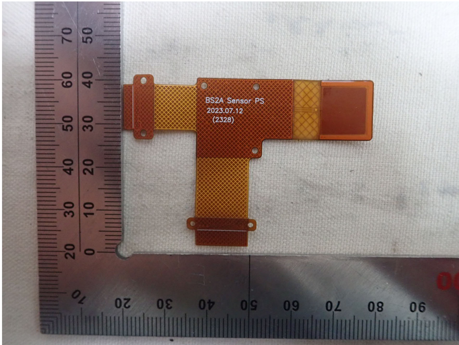
Sensor Film Front
