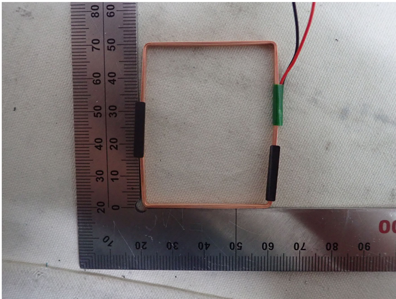
Coil Antenna Front
