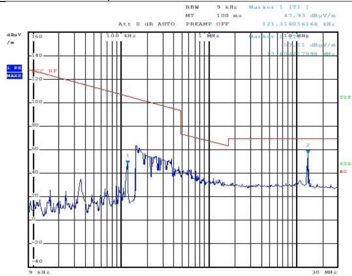
Radiated Spurious Emission 9 kHz – 30 MHz : LF ASK
