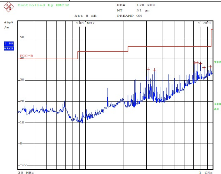
Radiated Spurious Emission 30 MHz – 1 GHz : LF ASK
