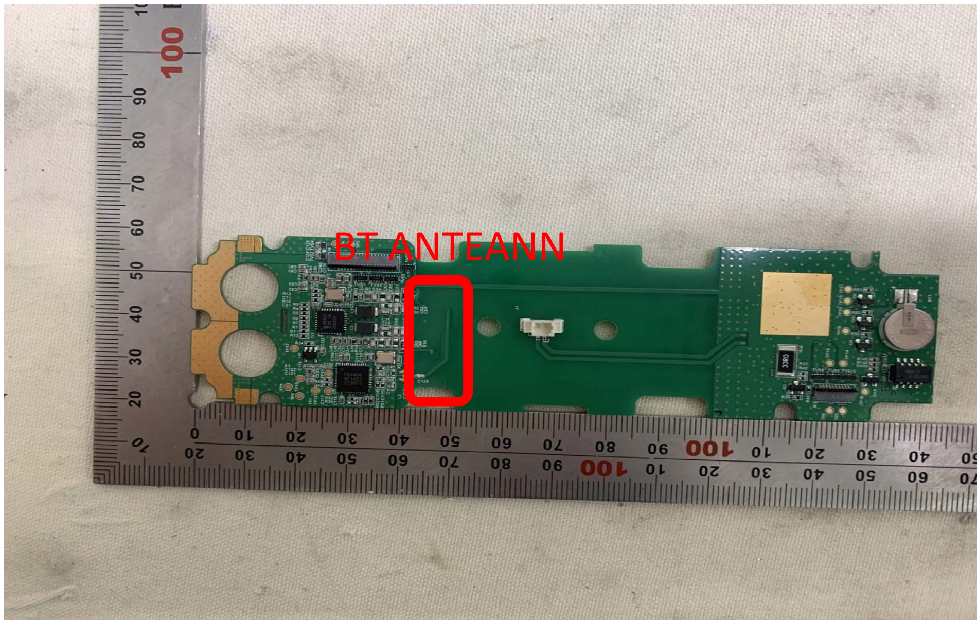
RF BOARD Front
