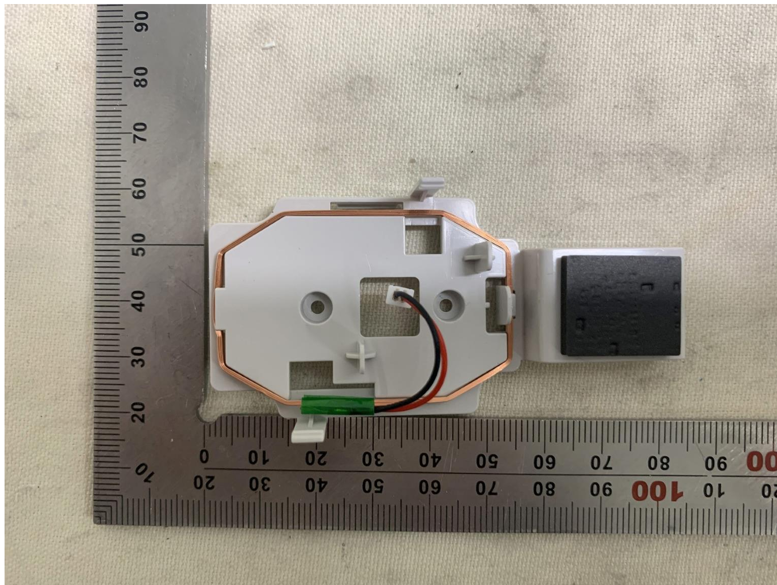
COIL ANTENNA
