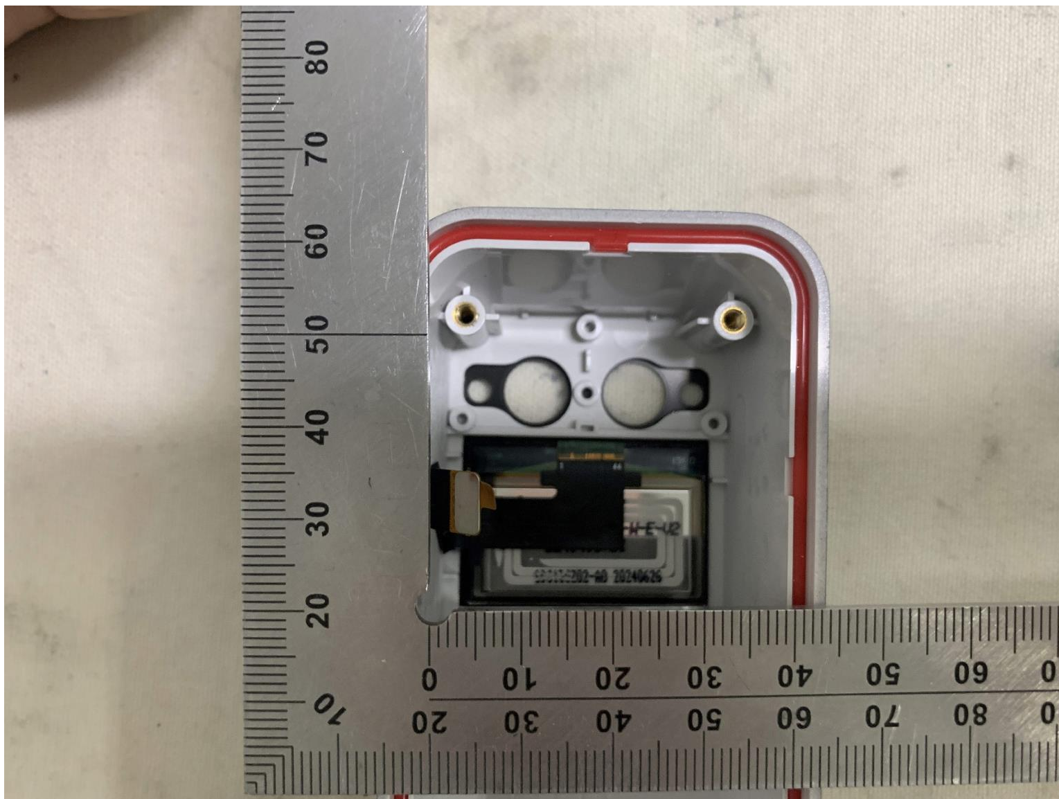
LCD Rear
