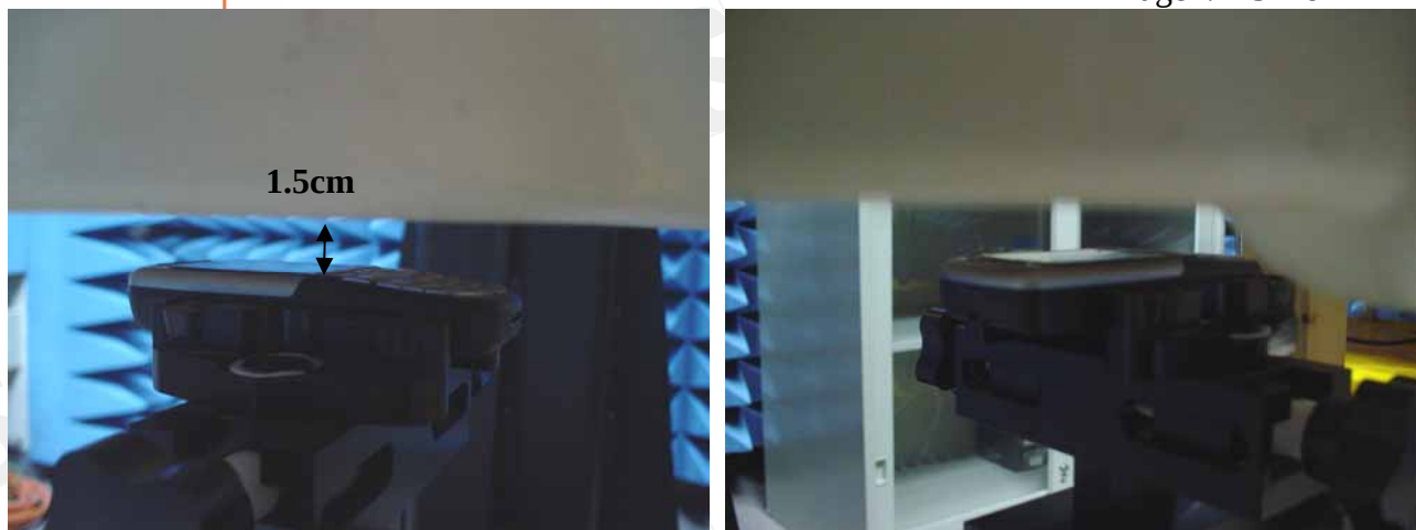
Fig.8 Body worn- EUT front to flat phantom (testing in GPRS Mode)
