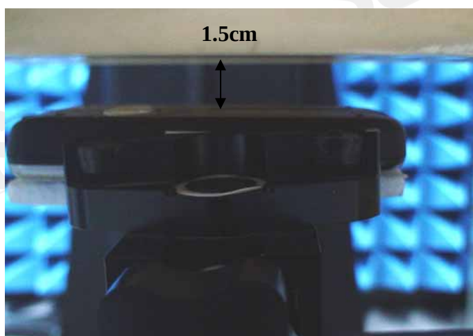
Fig.7 Body worn- EUT back to flat phantom (testing in GPRS Mode and Bluetooth OFF/ON)
