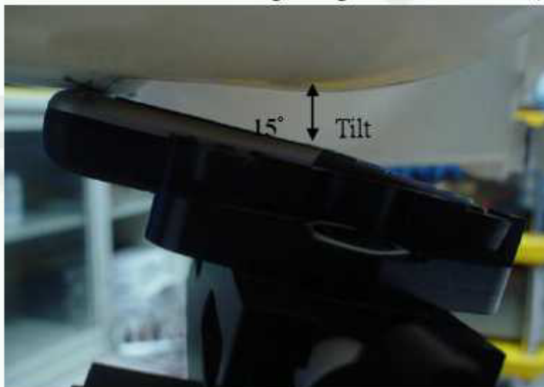
Fig.4 Right Head Section / Ear-Tilt Position(15°)
