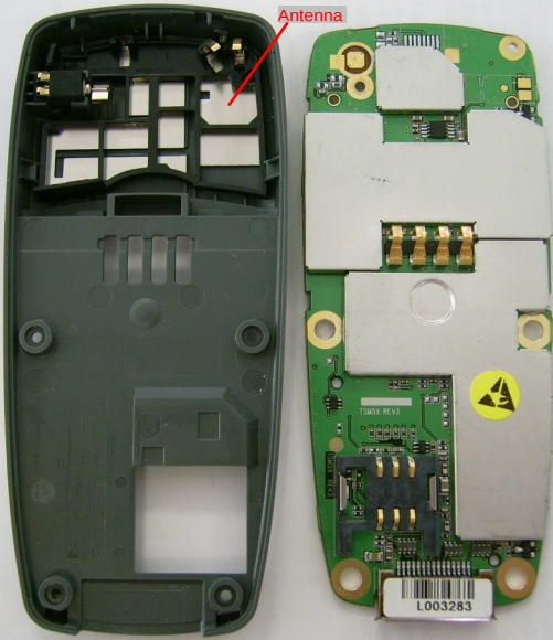
TSM2 PCB with shielding and antenna
