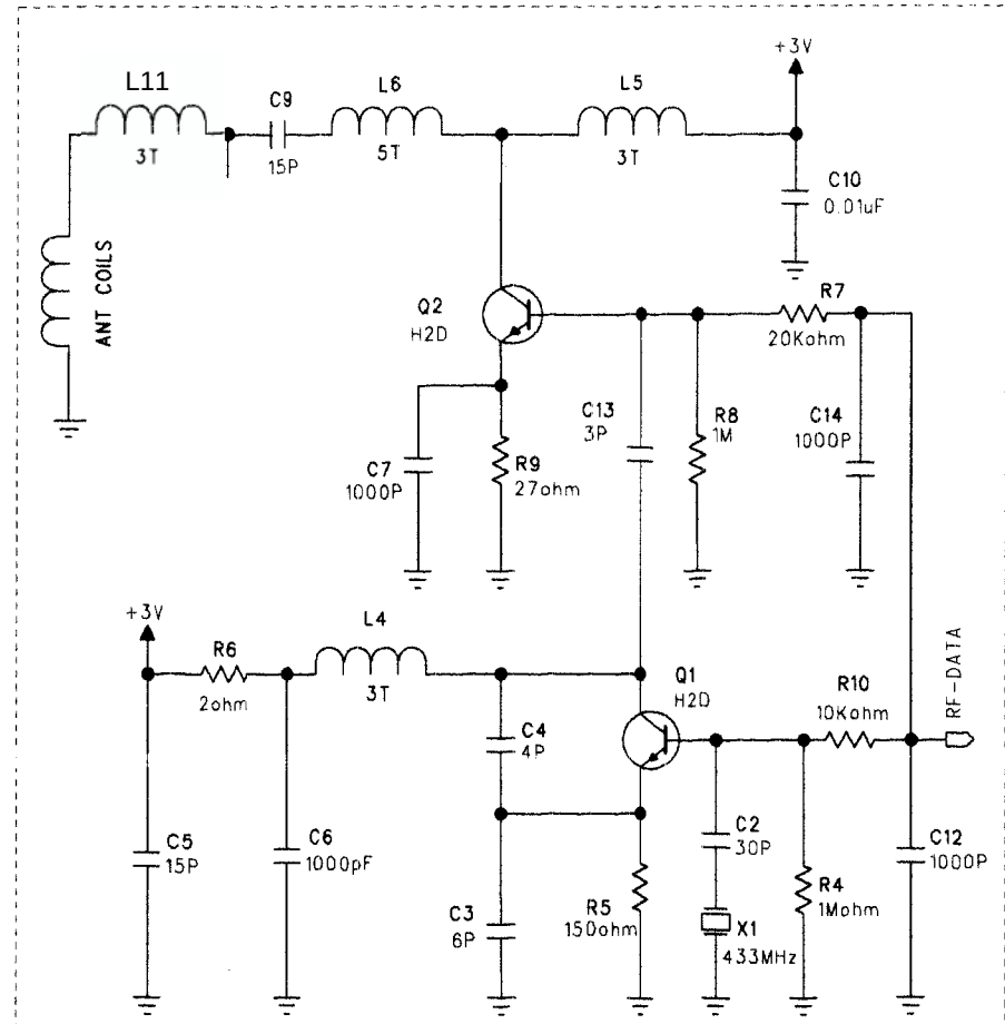
TRNSMIE BOARD.SCH
