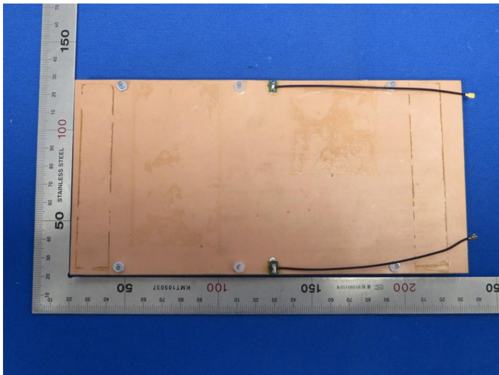
(8) EUT Photo (2.4GHz - 11dBi Antenna)
