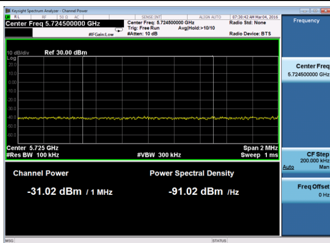
Band Edge – 20M 5755MHz (-17 eirp)
