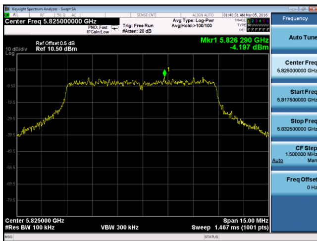
PSD – 10M 5825MHz Port A
