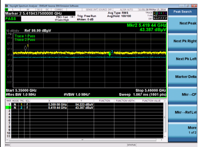
Higher Band 10M - 5240MHz
