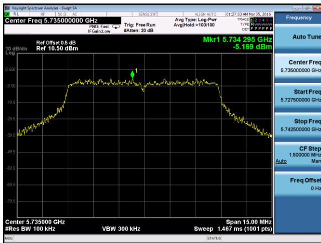
PSD – 10M 5735MHz Port A
