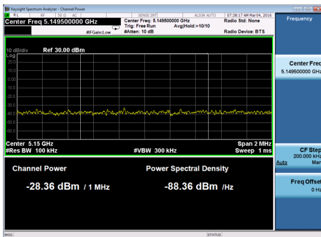
Band Edge – 40M 5190MHz
