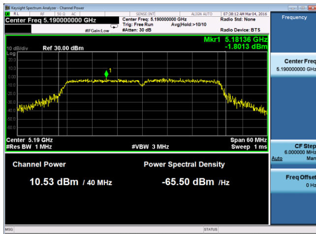
PSD – 40M 5190MHz Port A
