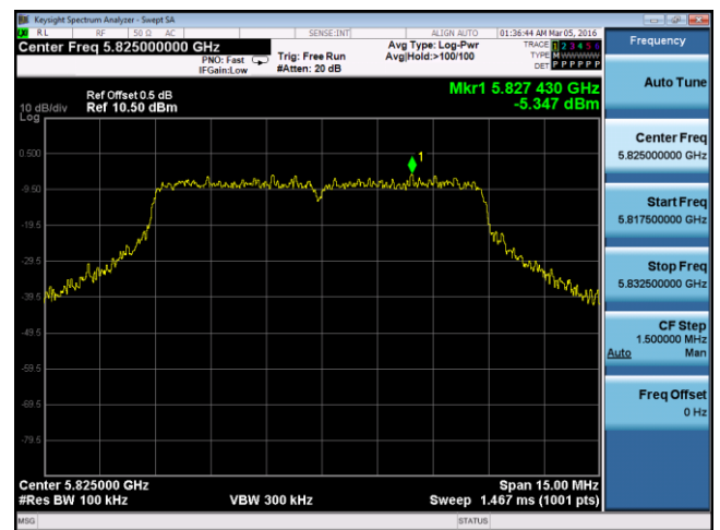
PSD – 10M 5825MHz Port B
