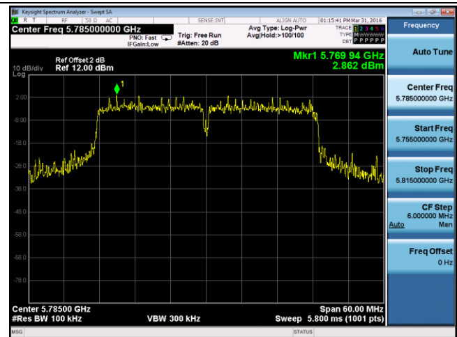
PSD – 40M 5785MHz Port B
