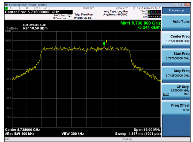
PSD – 10M 5735MHz Port B
