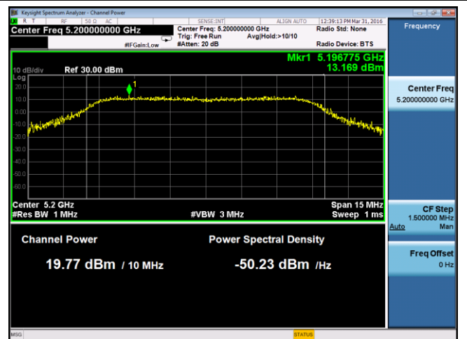
PSD – 10M 5200MHz Port B
