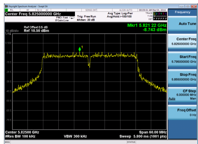
PSD – 40M 5825MHz Port B
