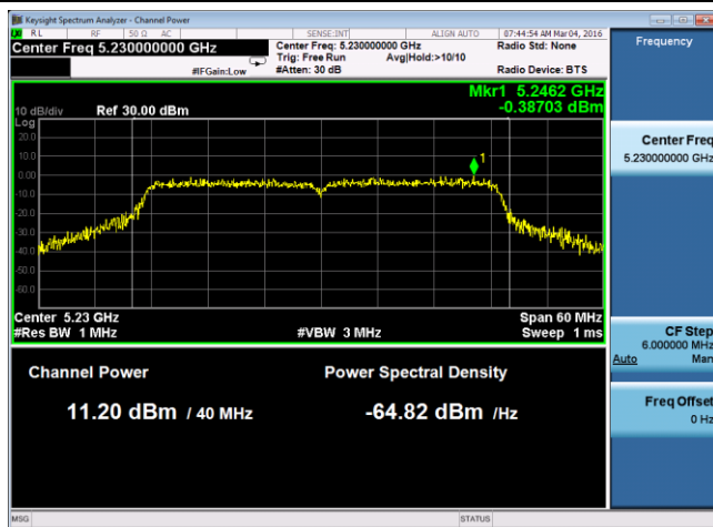
PSD – 40M 5230MHz Port A
