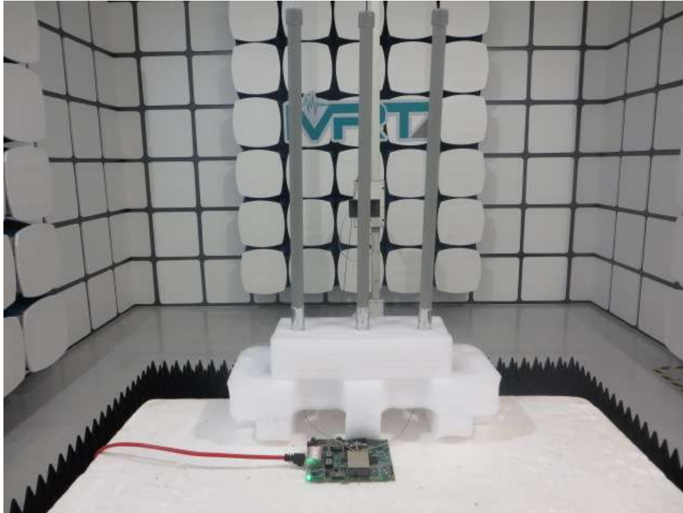
Description: Radiated Emission Test Setup for 18GHz ~ 40GHz for Panel Antenna 2#
