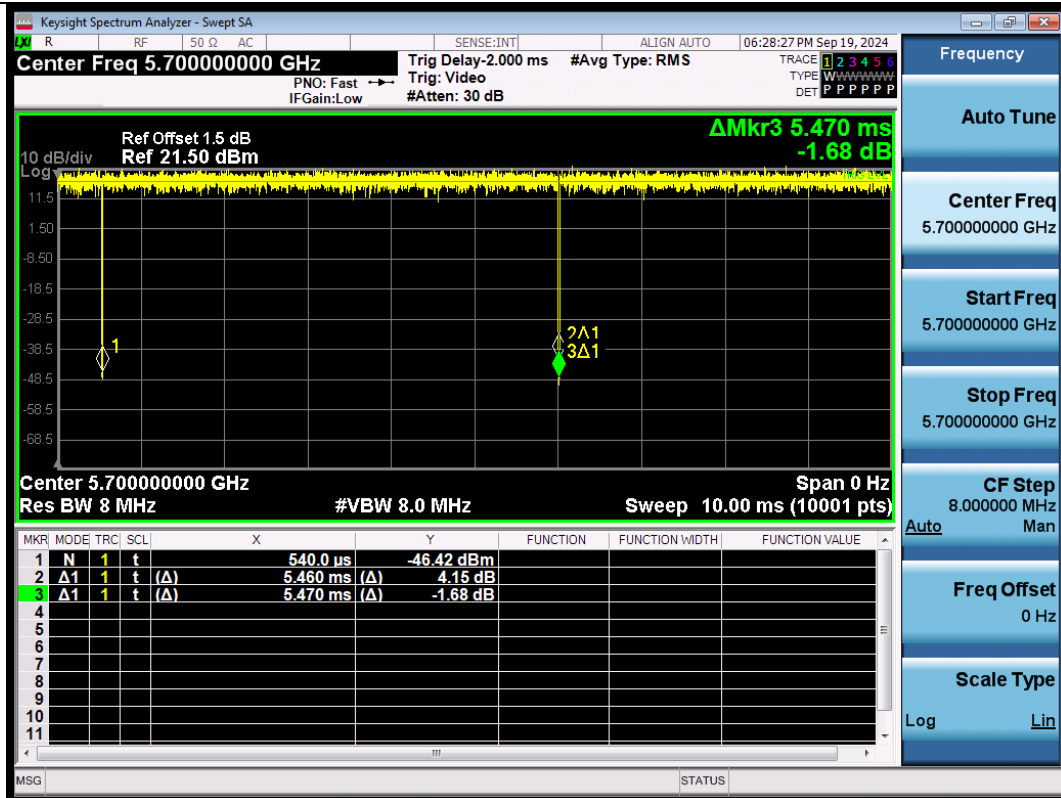
NTNV-11BE20SISO-Ant1-5700
