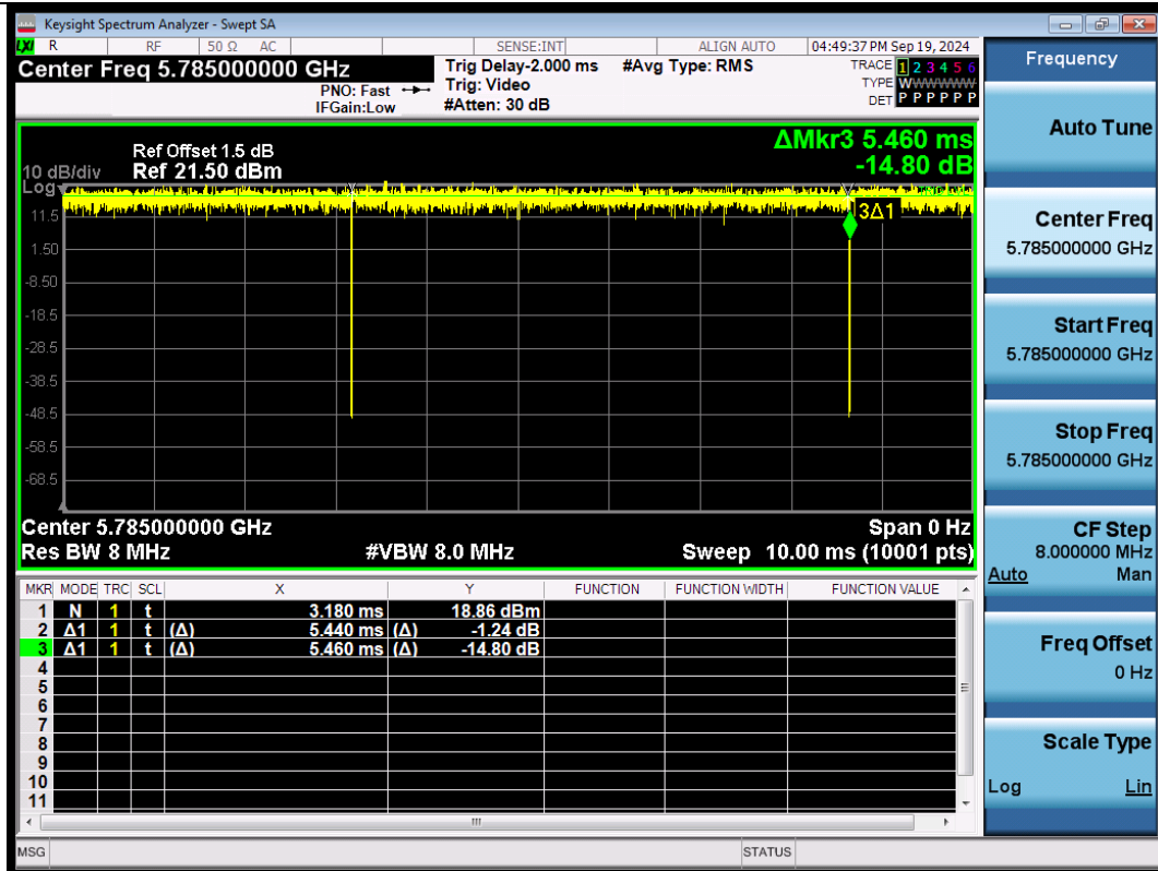
NTNV-11AX20SISO-Ant1-5785
