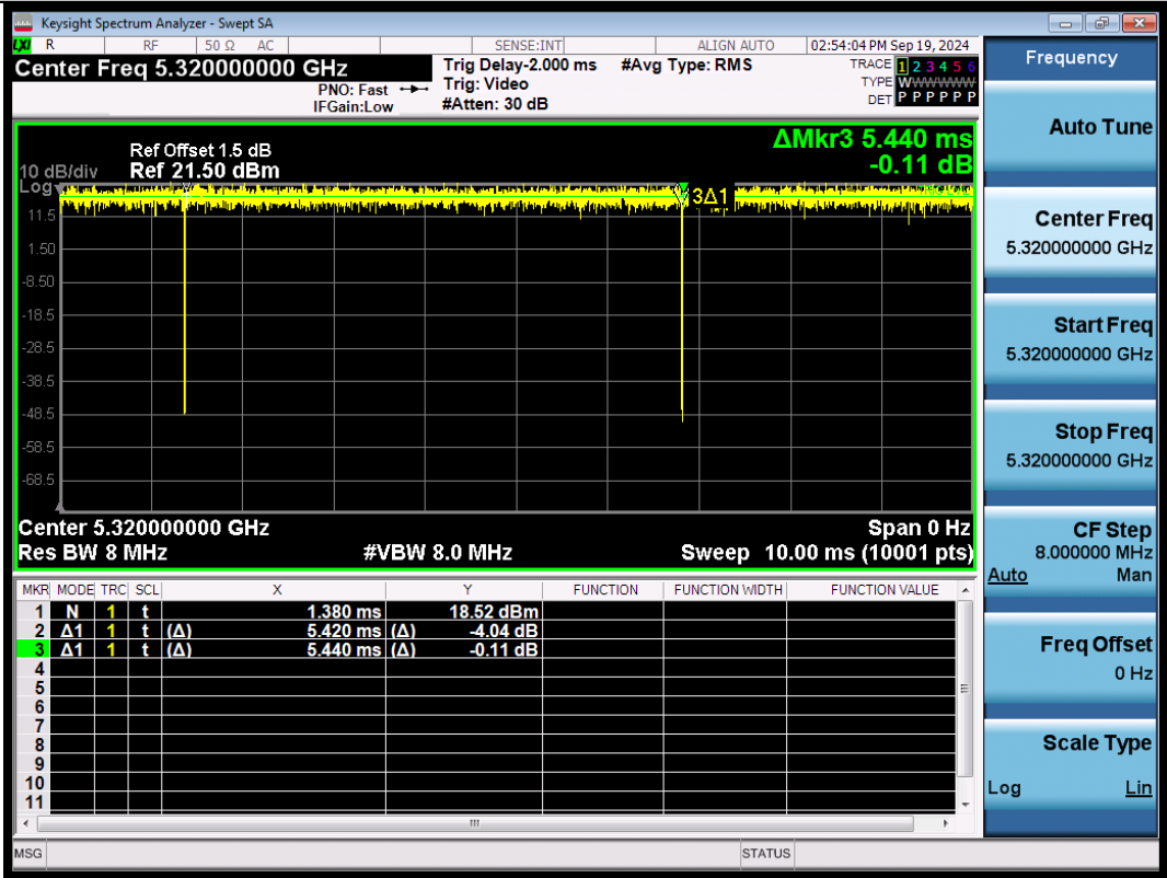
NTNV-11AC20SISO-Ant1-5320
