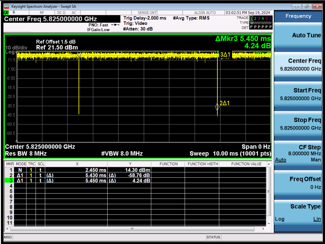
NTNV-11AC20SISO-Ant1-5825
