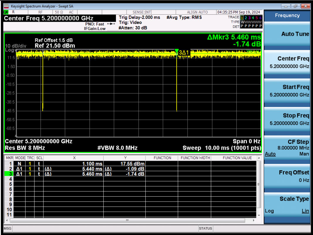
NTNV-11AX20SISO-Ant1-5200
