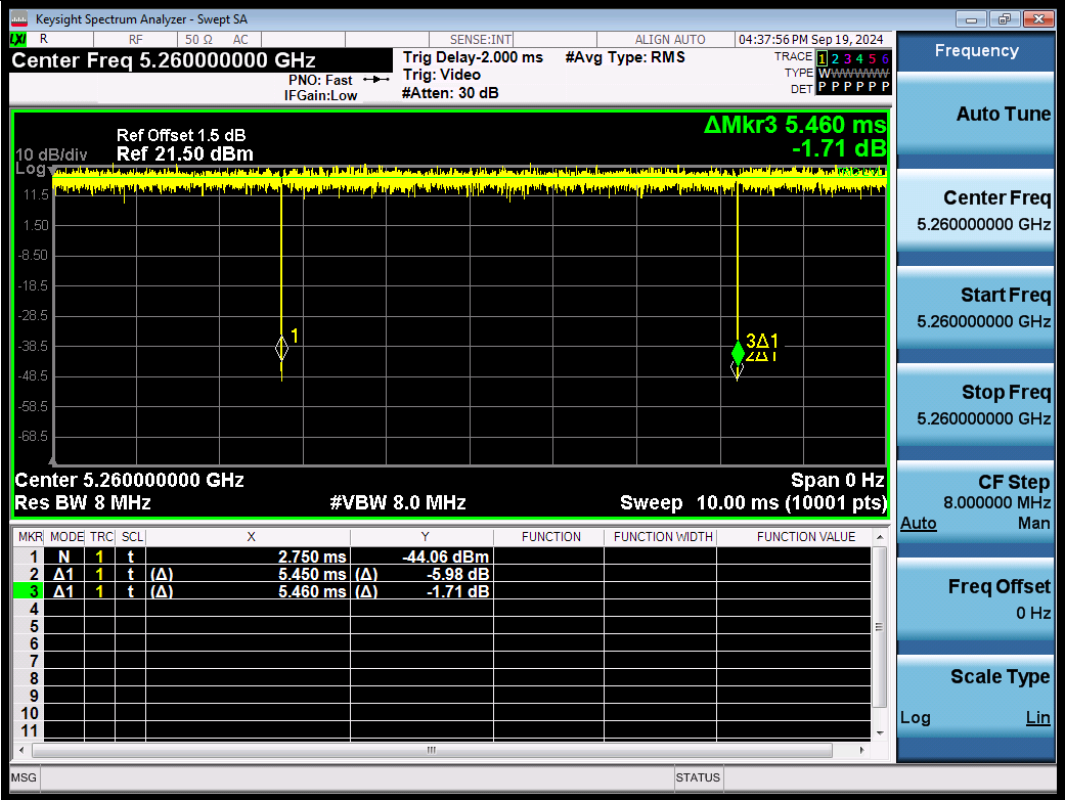
NTNV-11AX20SISO-Ant1-5260
