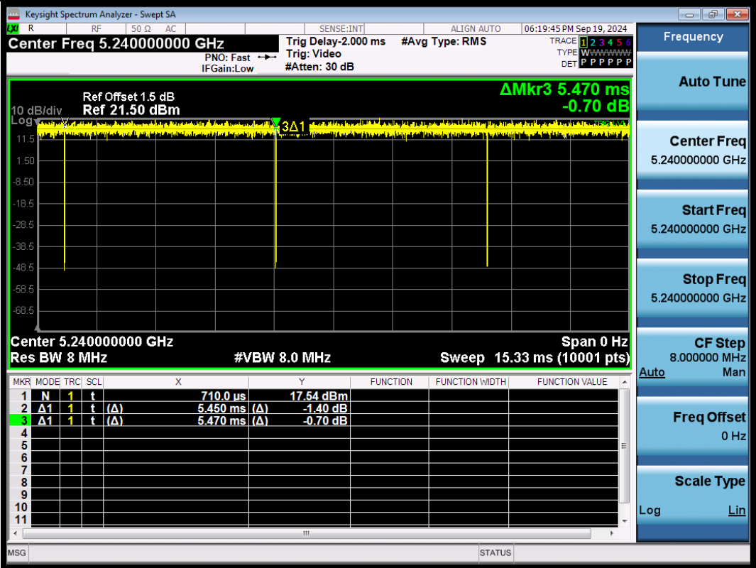
NTNV-11BE20SISO-Ant1-5240
