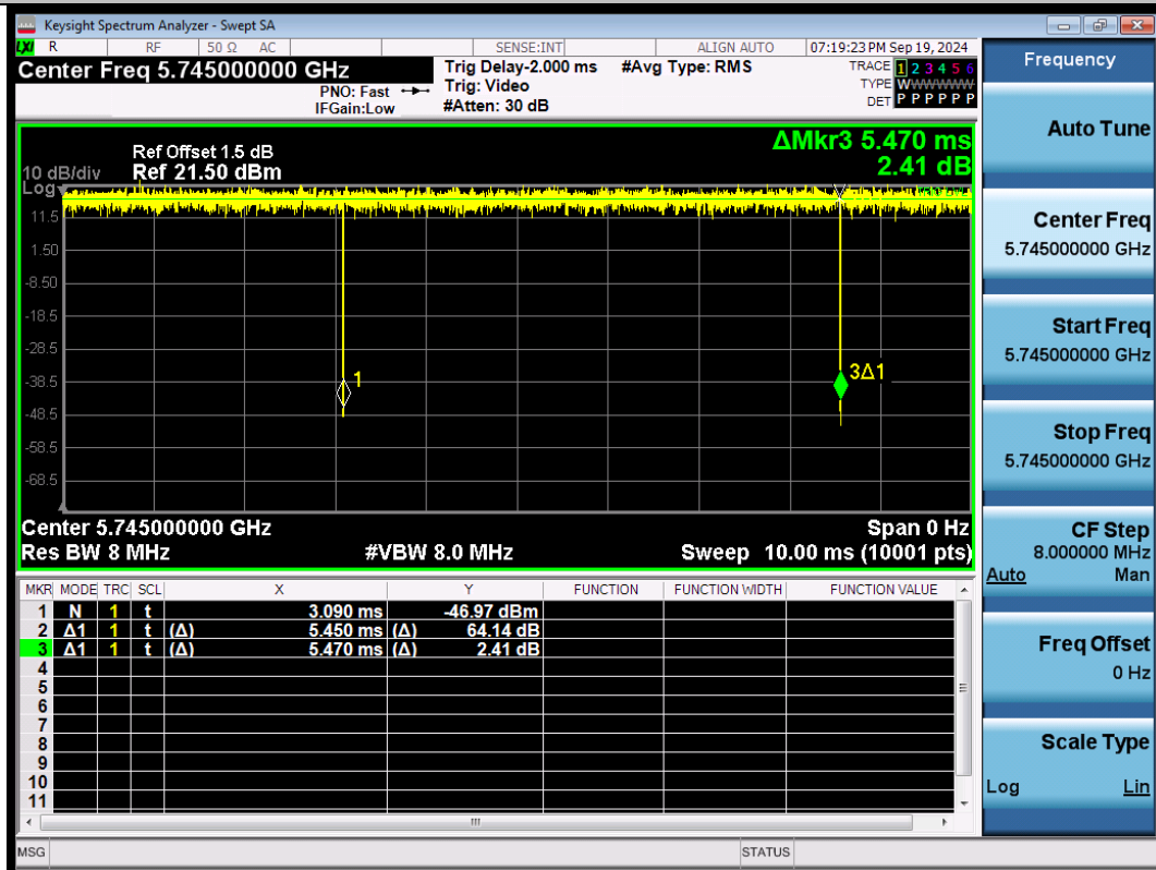
NTNV-11BE20SISO-Ant1-5745
