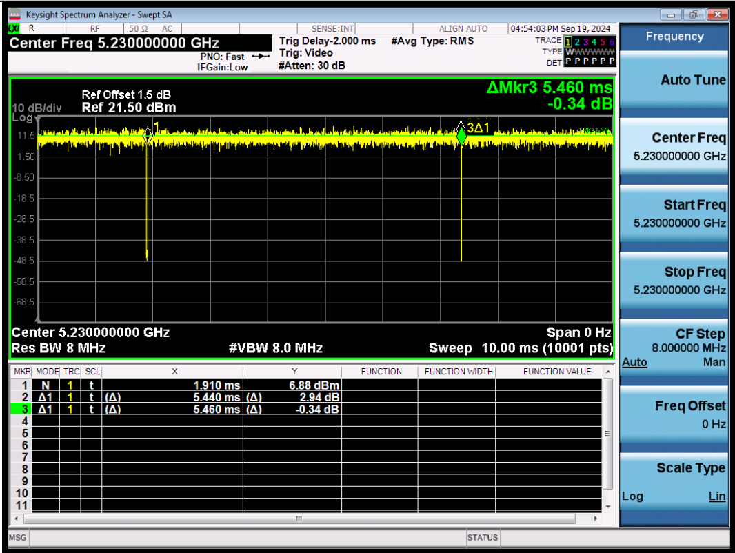
NTNV-11AX40SISO-Ant1-5230
