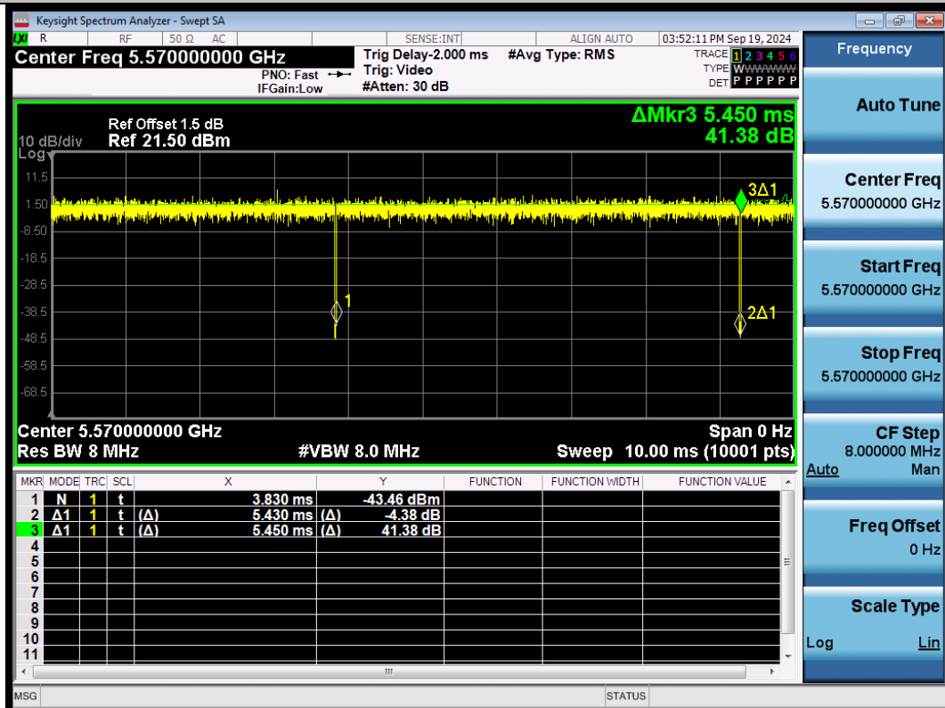
NTNV-11AC160SISO-Ant1-5570
