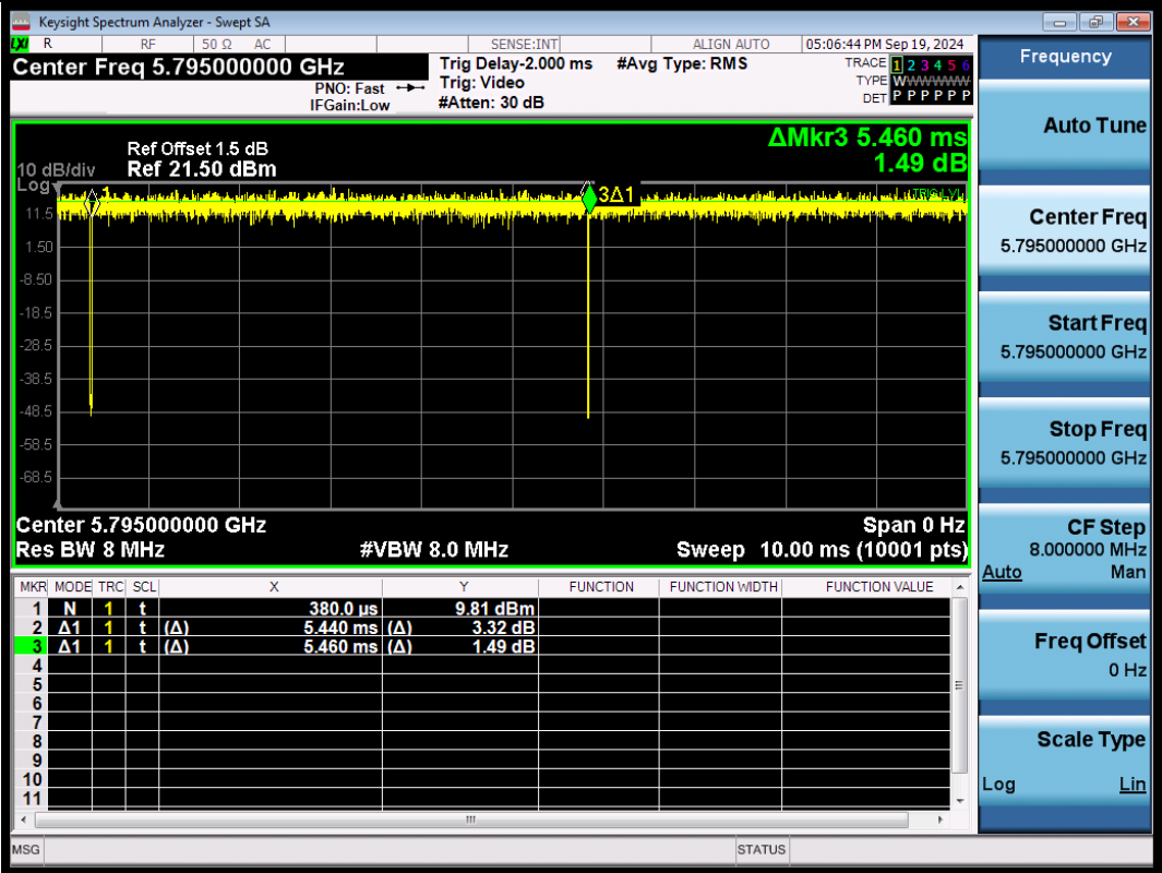
NTNV-11AX40SISO-Ant1-5795
