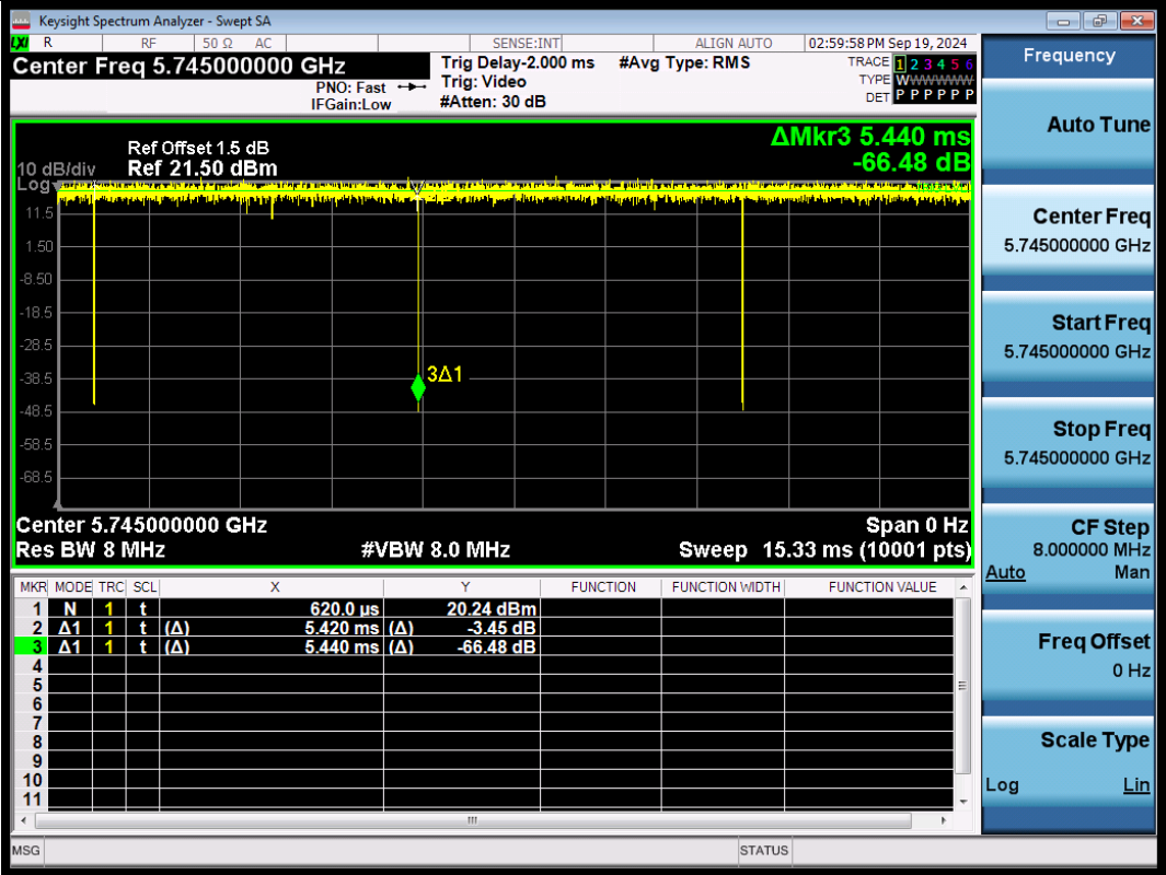
NTNV-11AC20SISO-Ant1-5745
