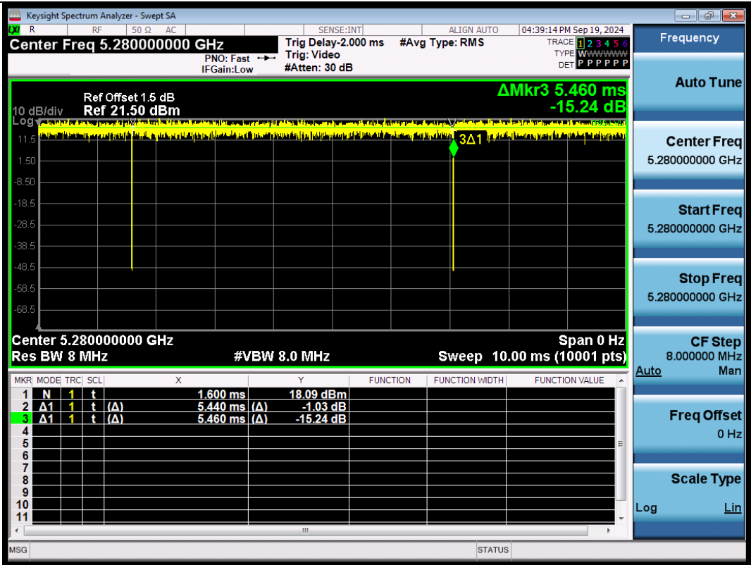
NTNV-11AX20SISO-Ant1-5280
