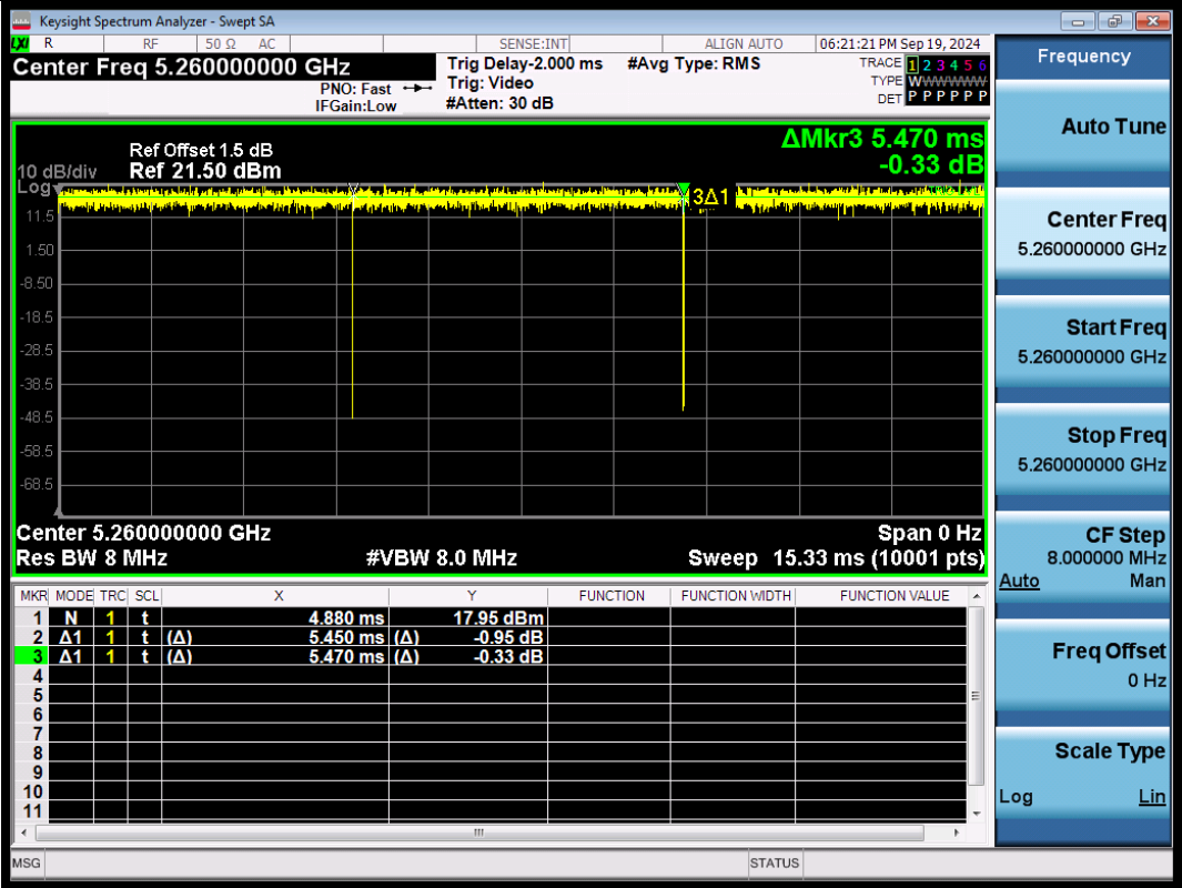
NTNV-11BE20SISO-Ant1-5260
