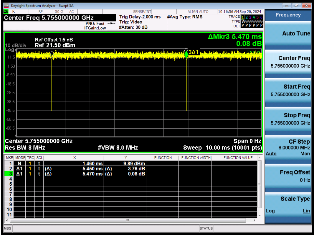
NTNV-11BE40SISO-Ant1-5755
