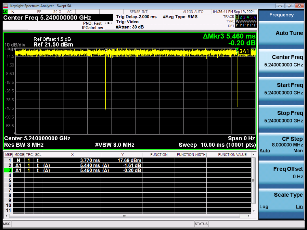
NTNV-11AX20SISO-Ant1-5240
