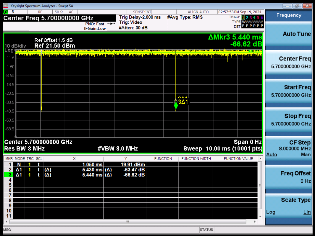
NTNV-11AC20SISO-Ant1-5700
