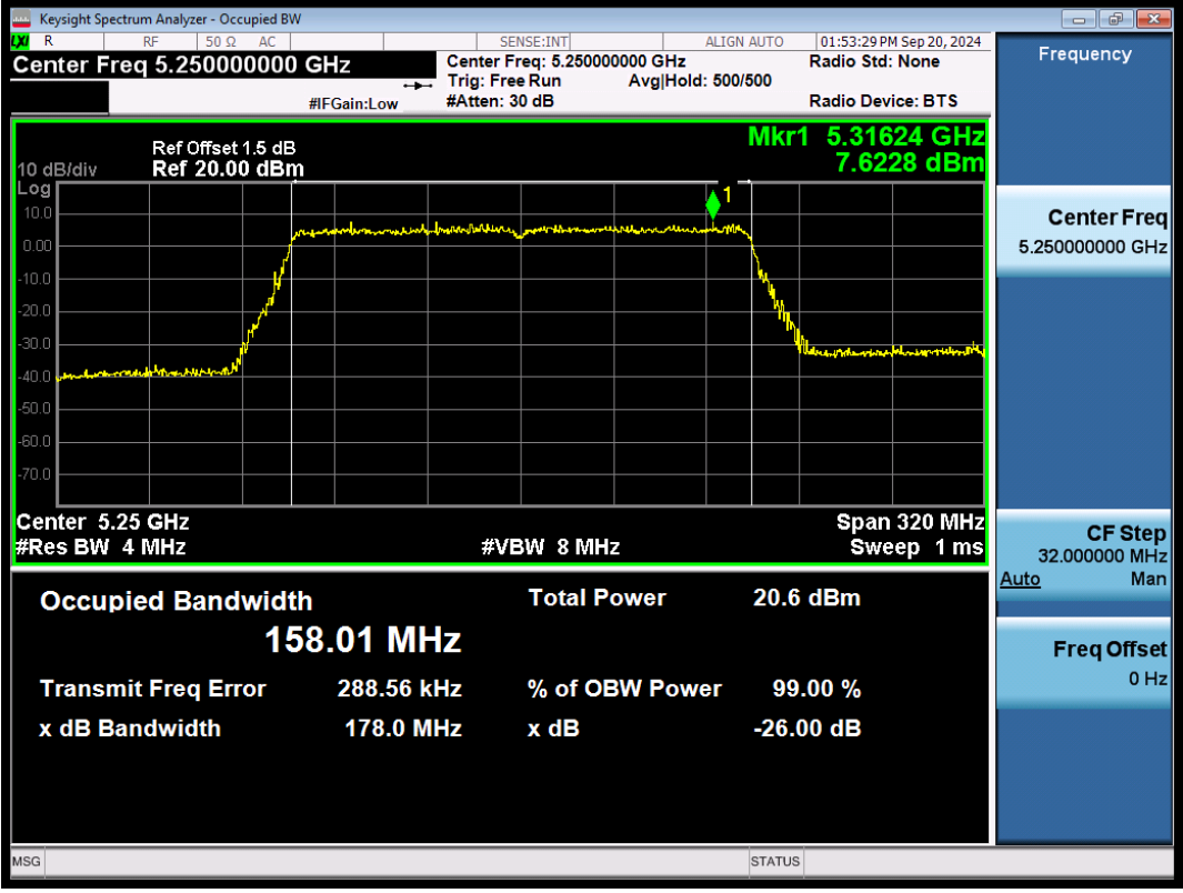
11BE160SISO-Ant1-5250
