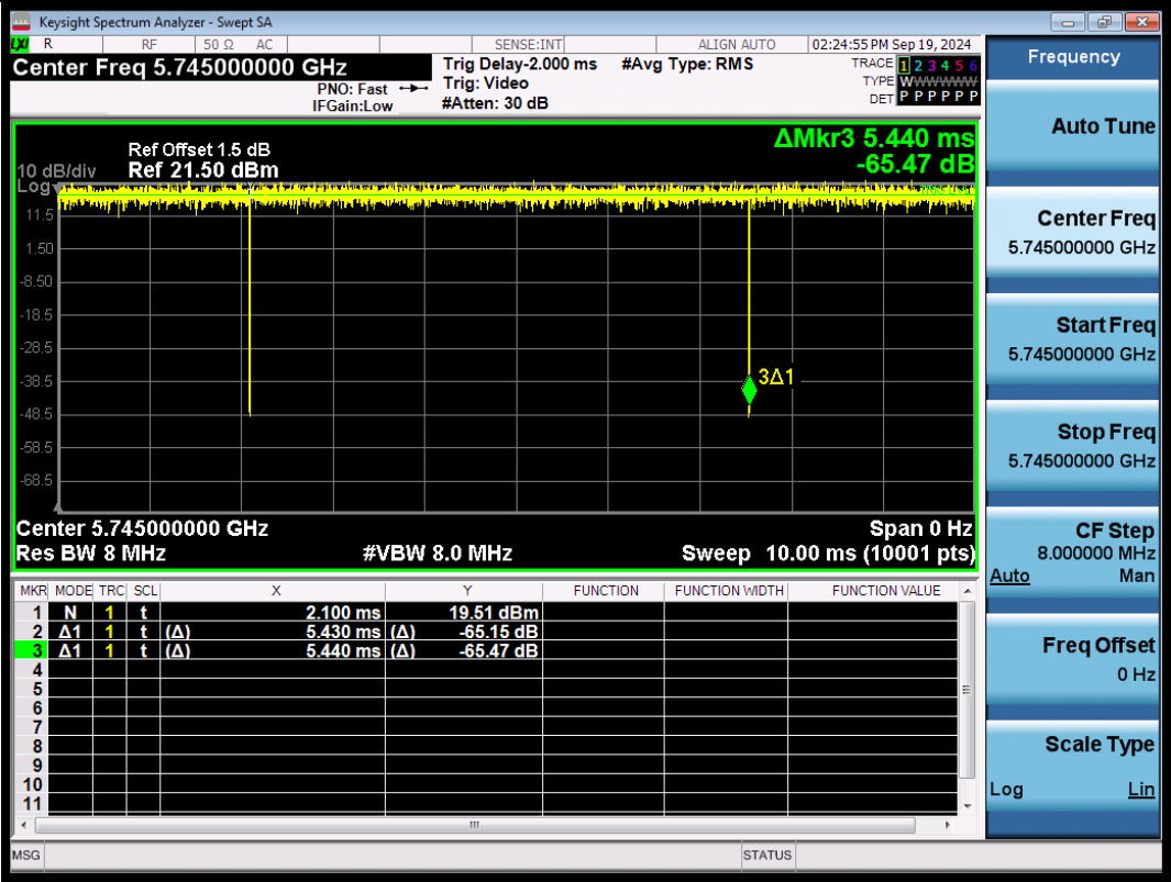
NTNV-11N20SISO-Ant1-5745
