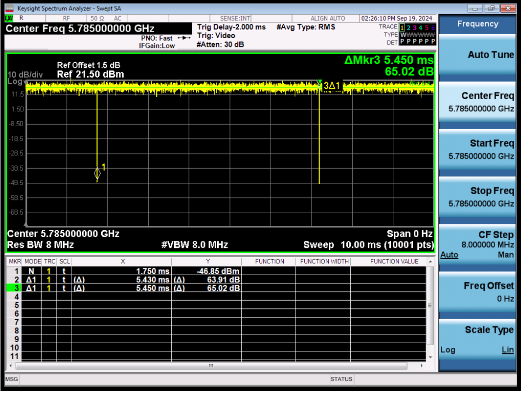
NTNV-11N20SISO-Ant1-5785
