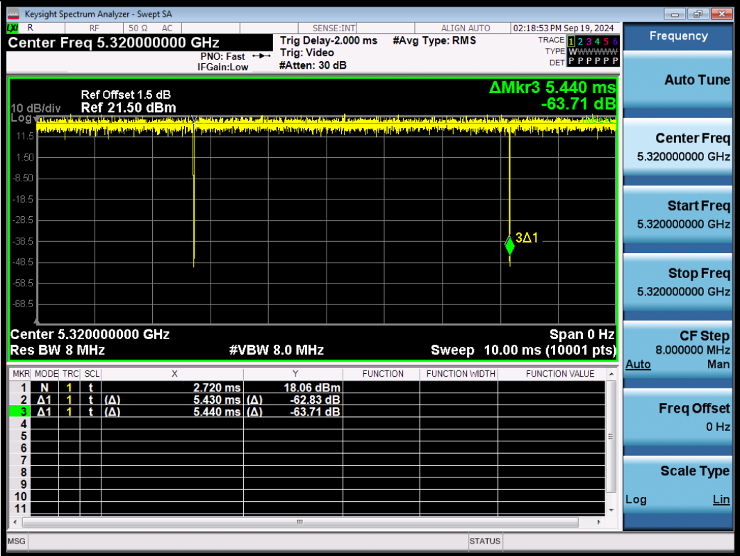
NTNV-11N20SISO-Ant1-5320
