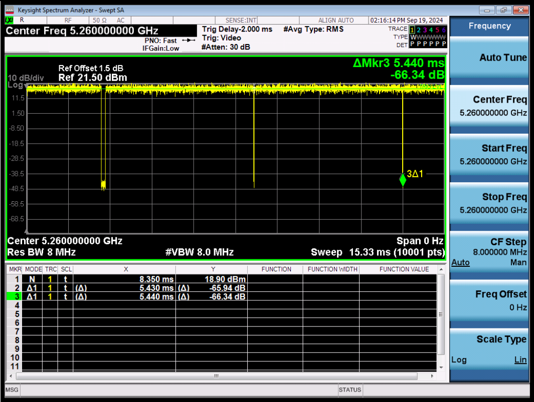
NTNV-11N20SISO-Ant1-5260
