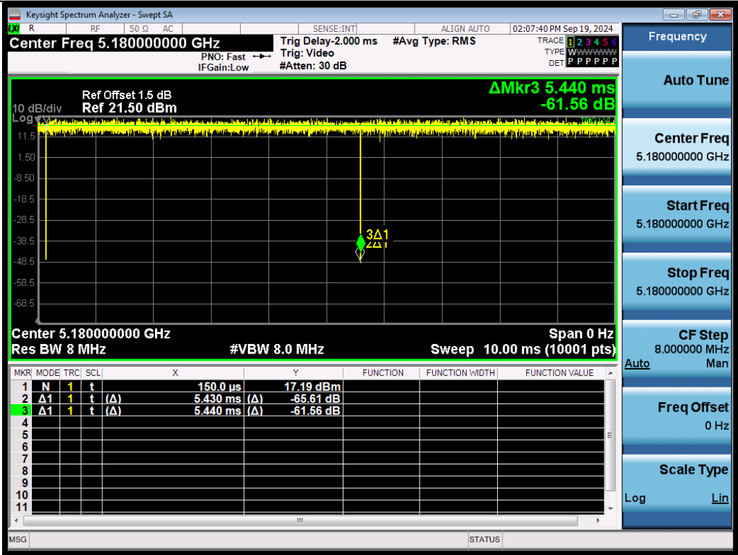
NTNV-11N20SISO-Ant1-5180
