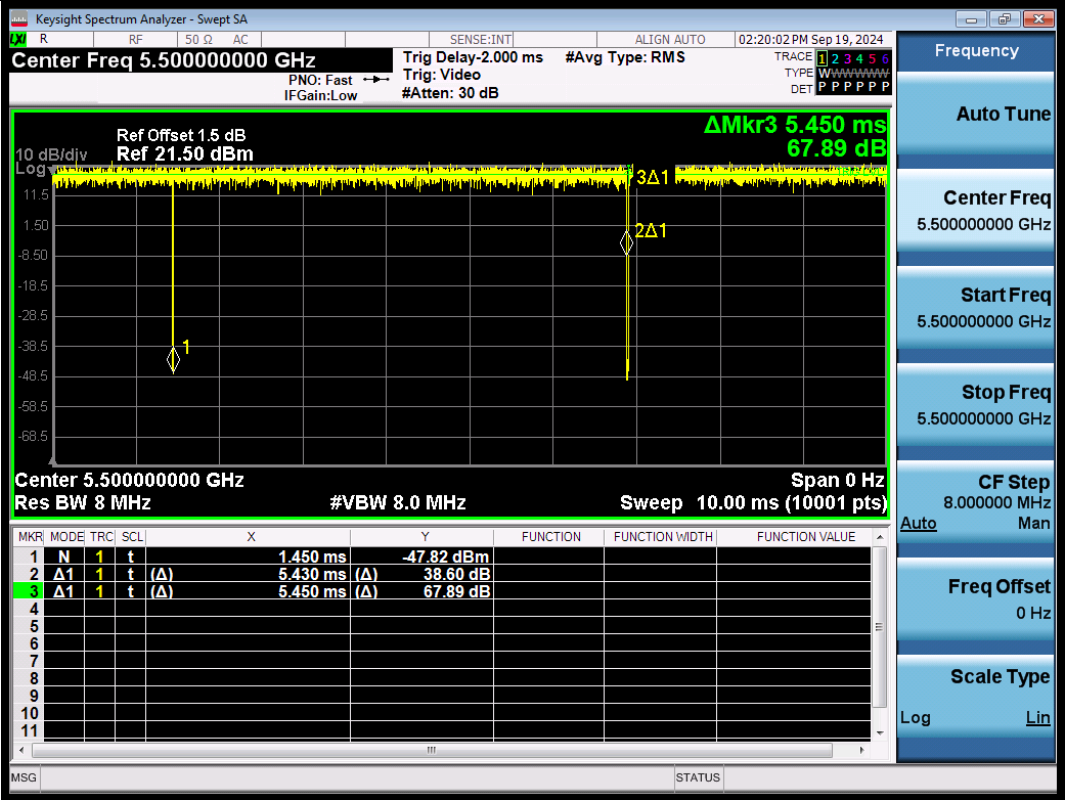
NTNV-11N20SISO-Ant1-5500
