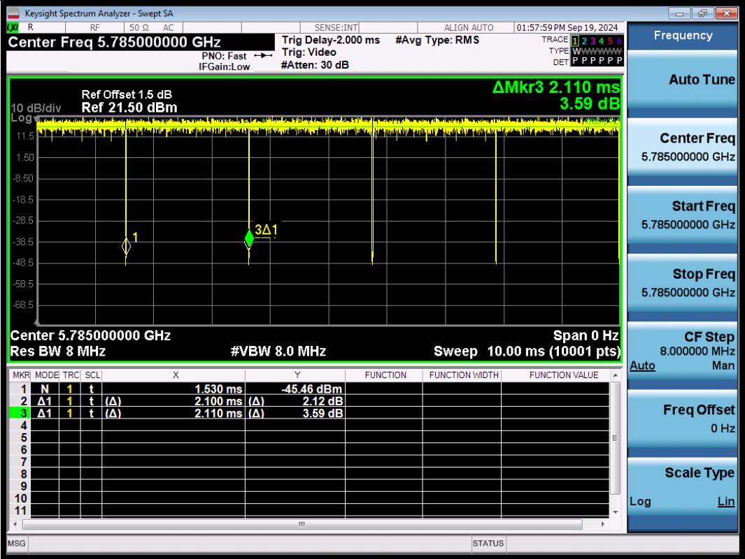
NTNV-11A-Ant1-5785
