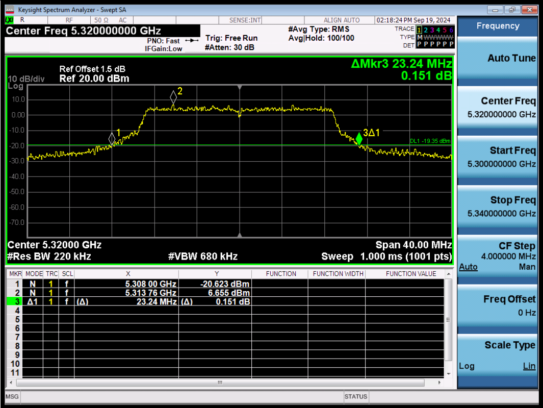
11N20SISO-Ant1-5320
