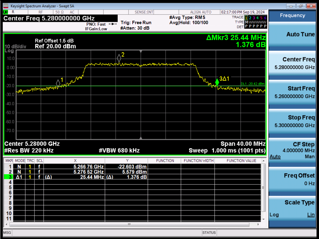
11N20SISO-Ant1-5280
