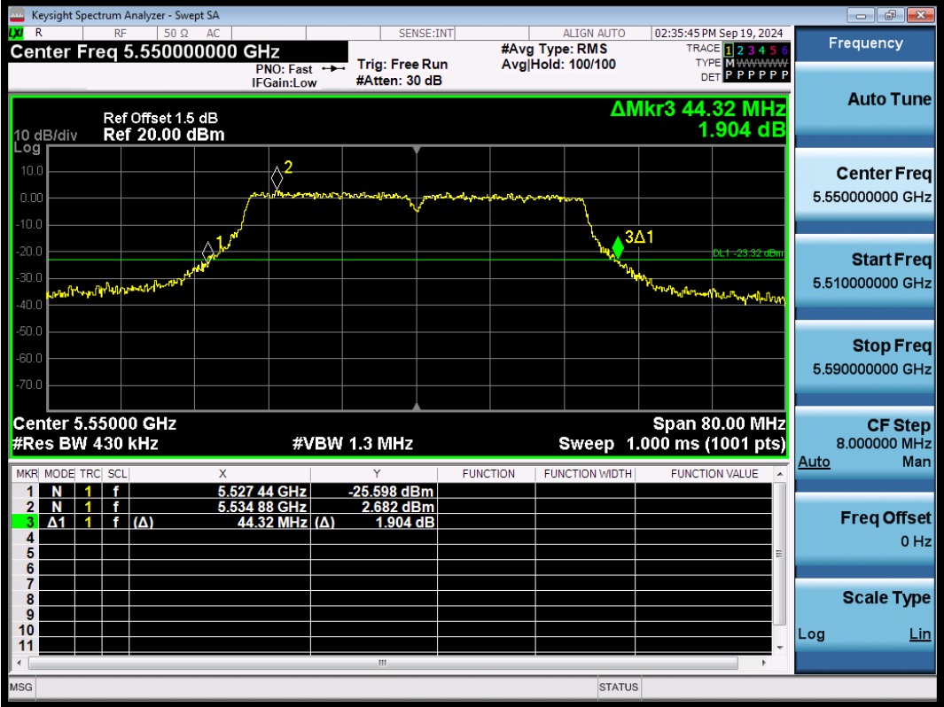
11N40SISO-Ant1-5550
