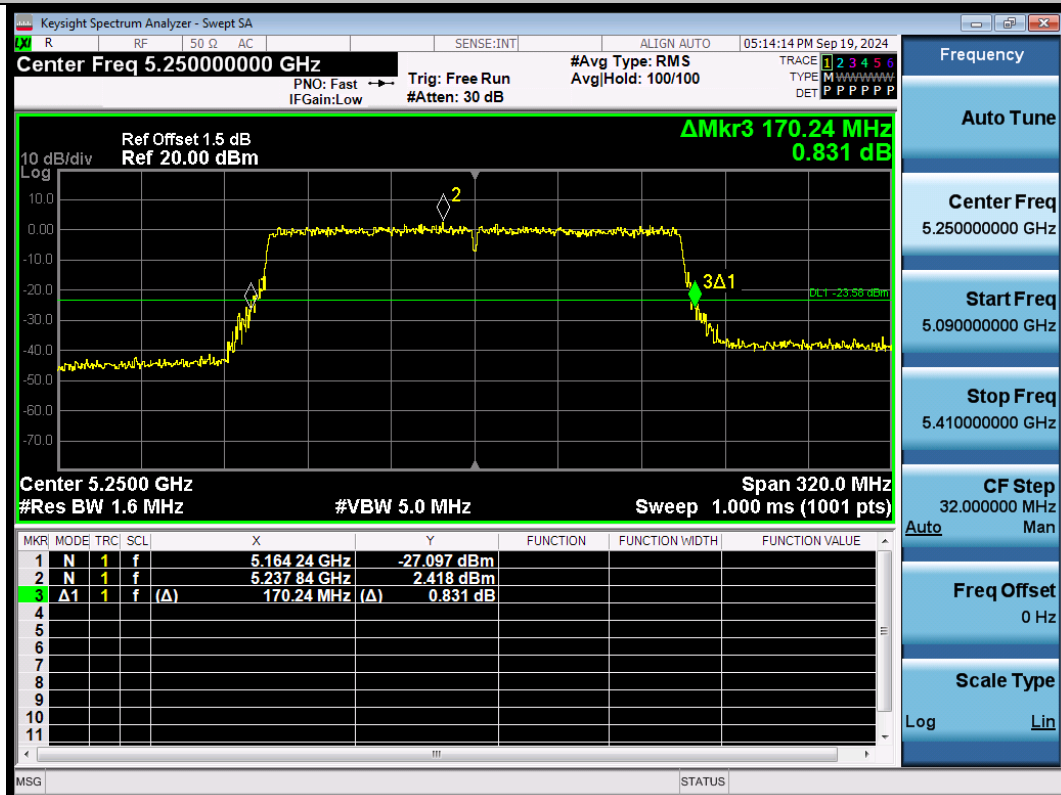
11AX160SISO-Ant1-5250
