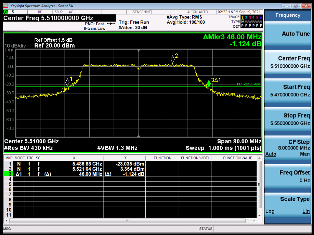
11N40SISO-Ant1-5510
