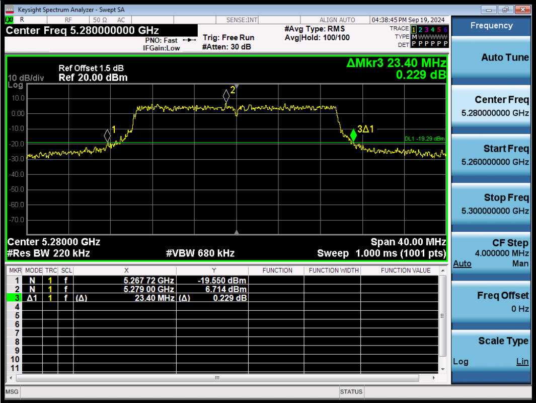
11AX20SISO-Ant1-5280
