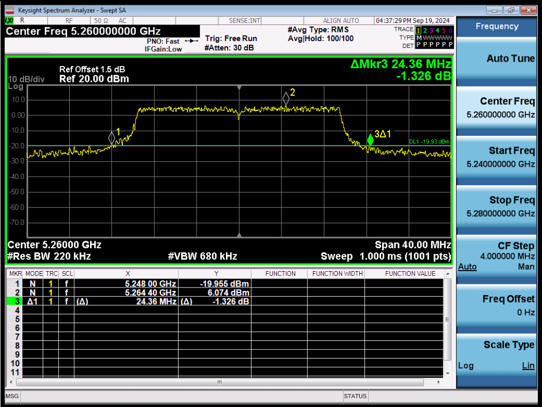
11AX20SISO-Ant1-5260
