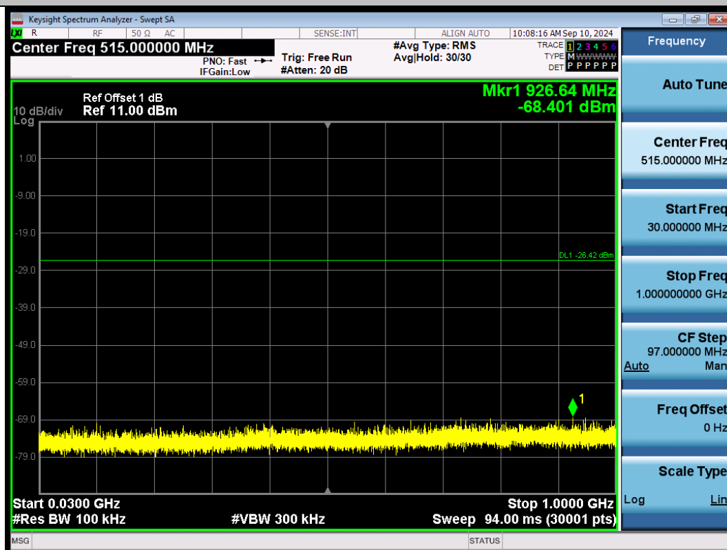
11AX20SISO-Ant1-2412-30~1000-PASS
