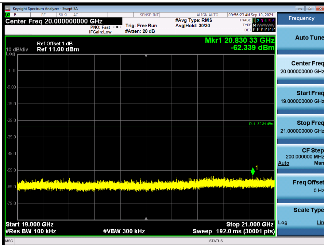
11N40SISO-Ant1-2452-19000~21000-PASS
