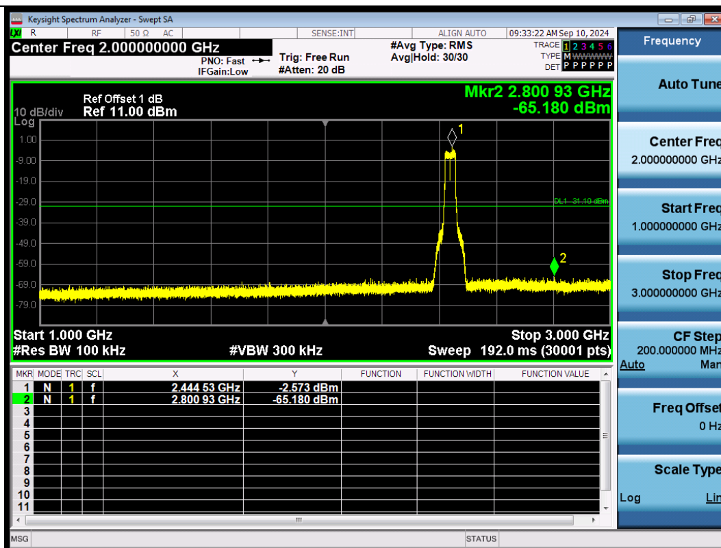
11N40SISO-Ant1-2437-1000~3000-PASS
