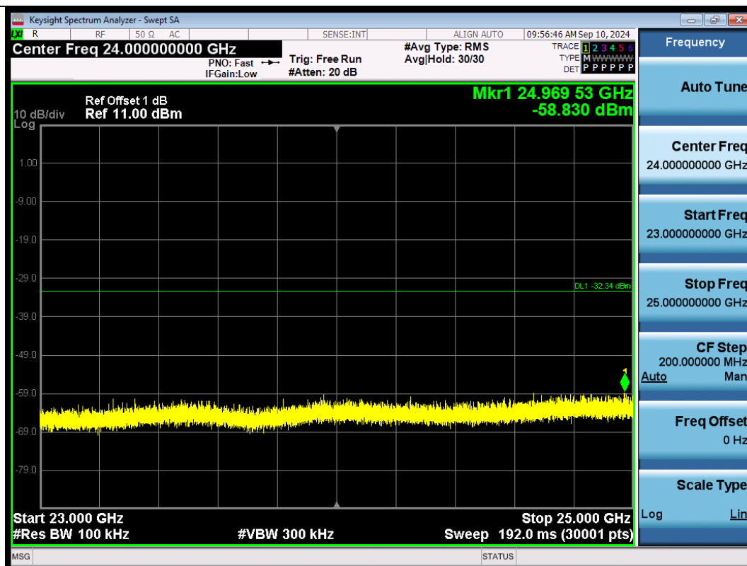
11N40SISO-Ant1-2452-23000~25000-PASS
