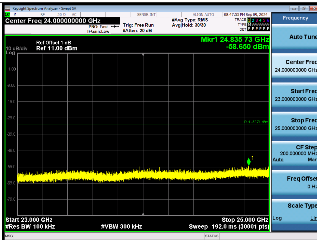
11N40SISO-Ant1-2422-23000~25000-PASS
