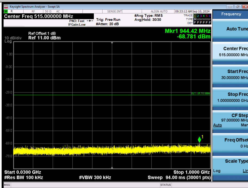
11N40SISO-Ant1-2437-30~1000-PASS
