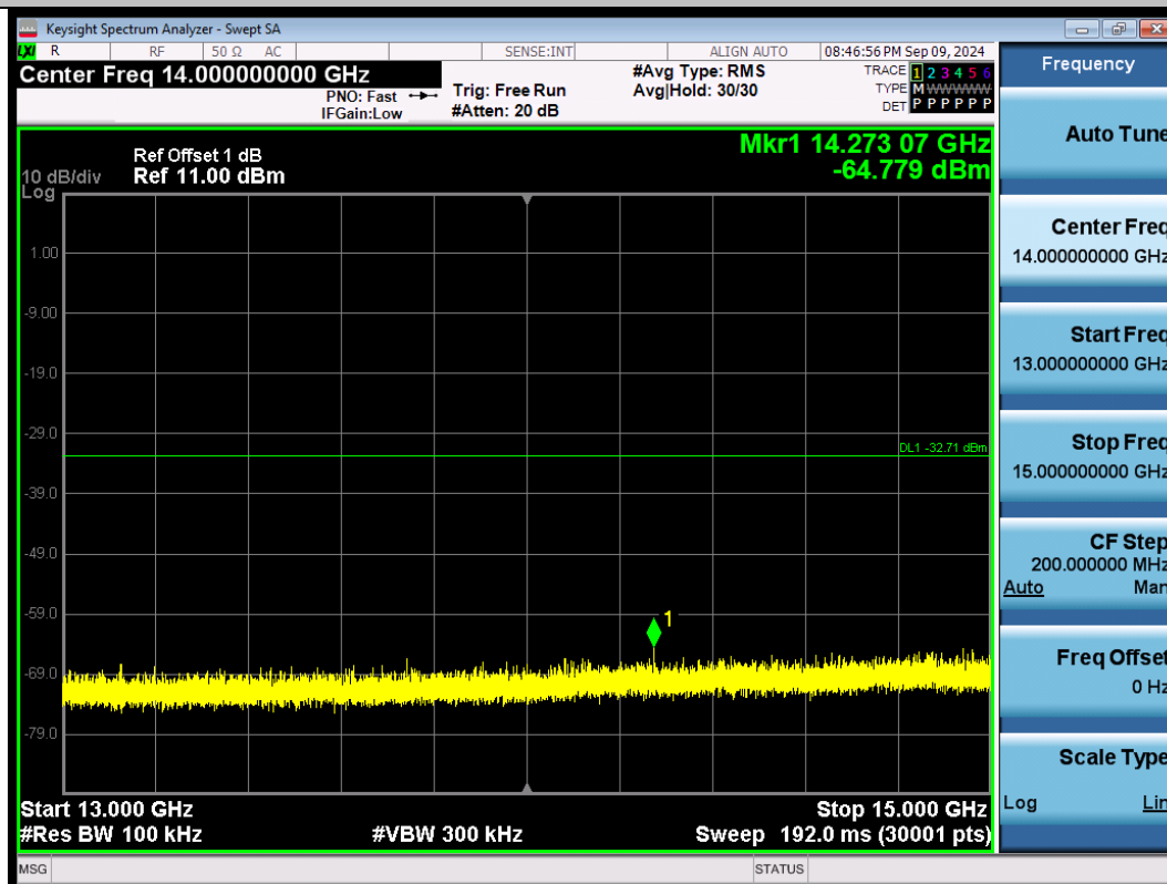
11N40SISO-Ant1-2422-13000~15000-PASS
