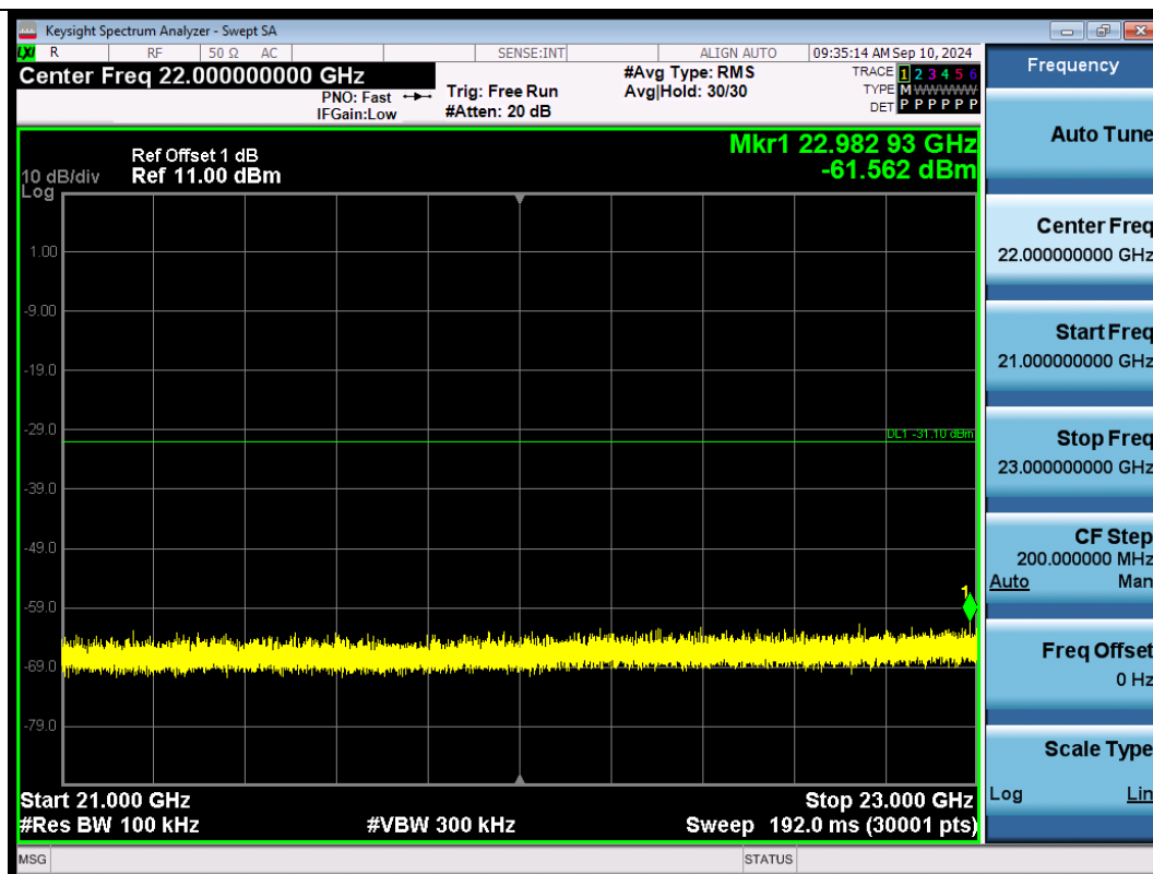
11N40SISO-Ant1-2437-21000~23000-PASS
