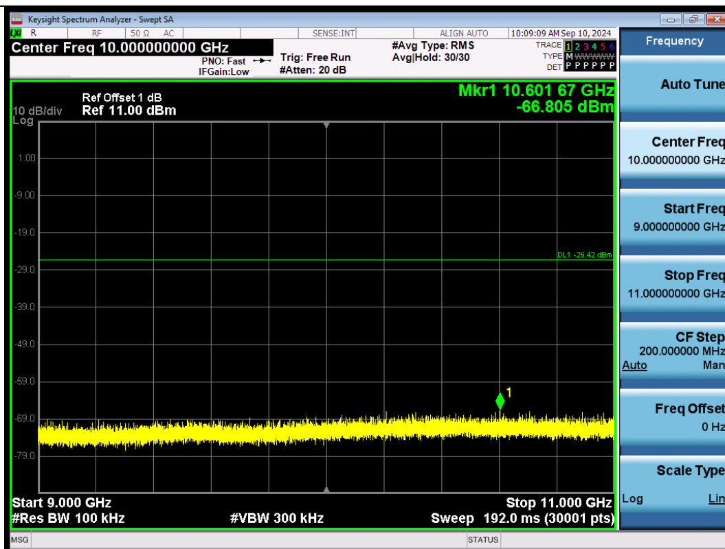
11AX20SISO-Ant1-2412-9000~11000-PASS
