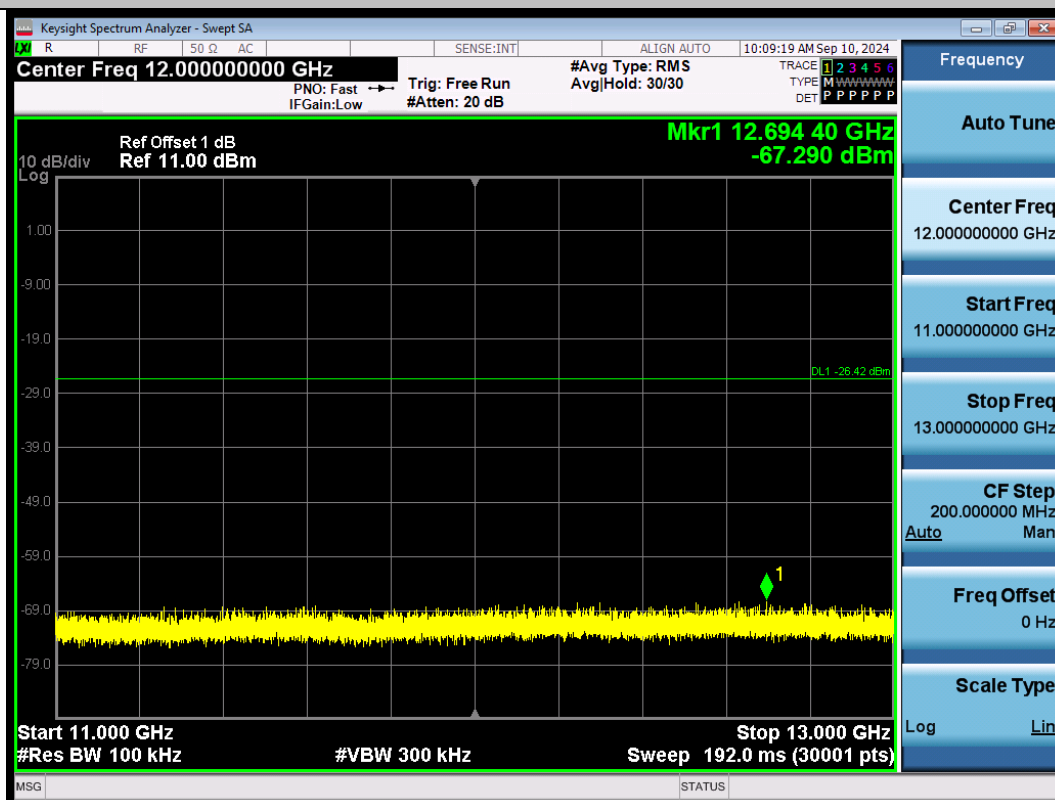
11AX20SISO-Ant1-2412-11000~13000-PASS
