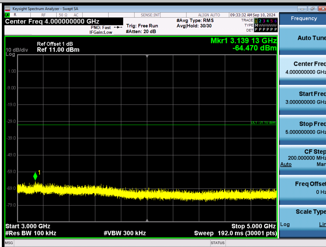
11N40SISO-Ant1-2437-3000~5000-PASS
