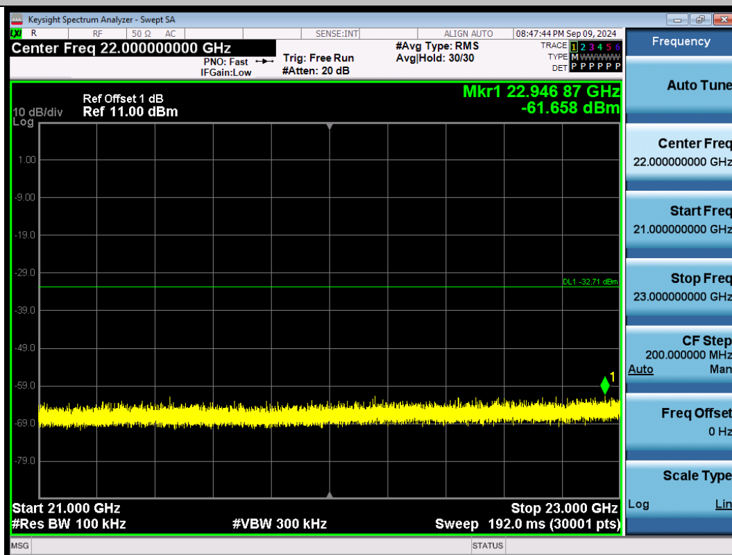
11N40SISO-Ant1-2422-21000~23000-PASS
