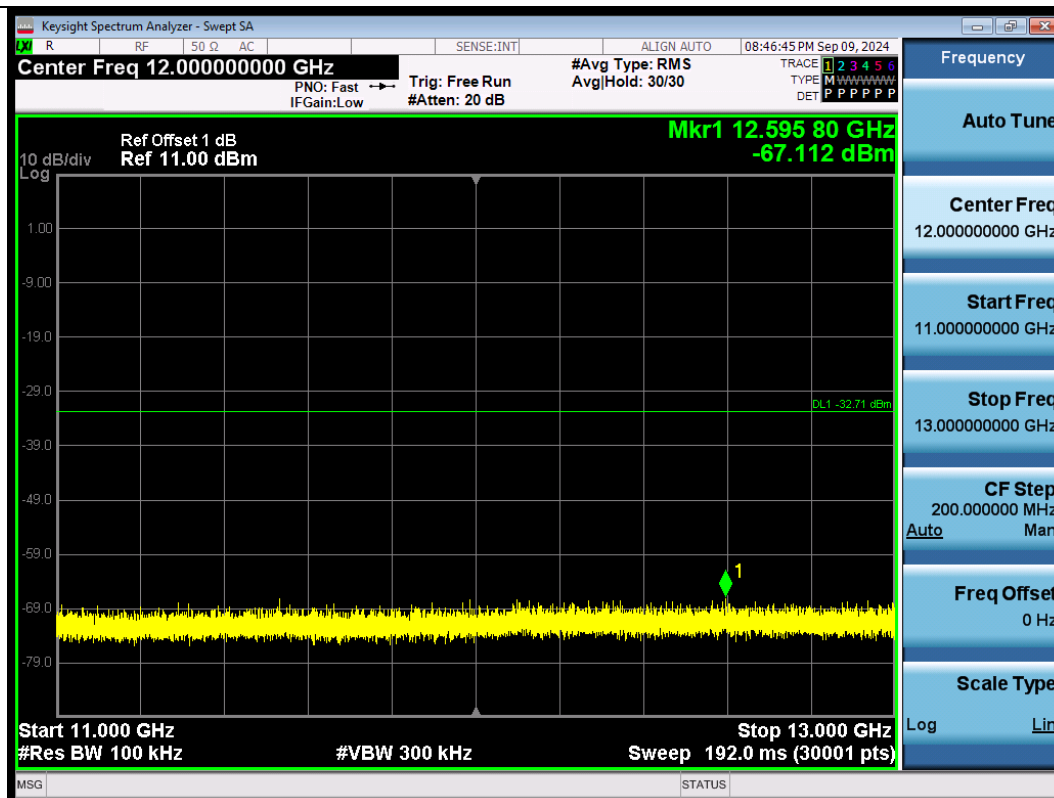
11N40SISO-Ant1-2422-11000~13000-PASS
