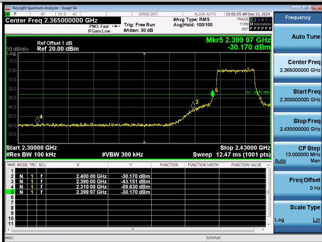
11AX20SISO-Ant1-2412-PASS
