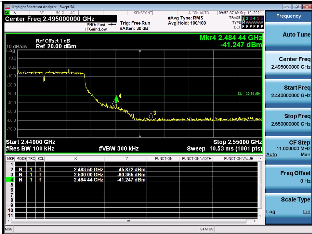
11N40SISO-Ant1-2452-PASS
