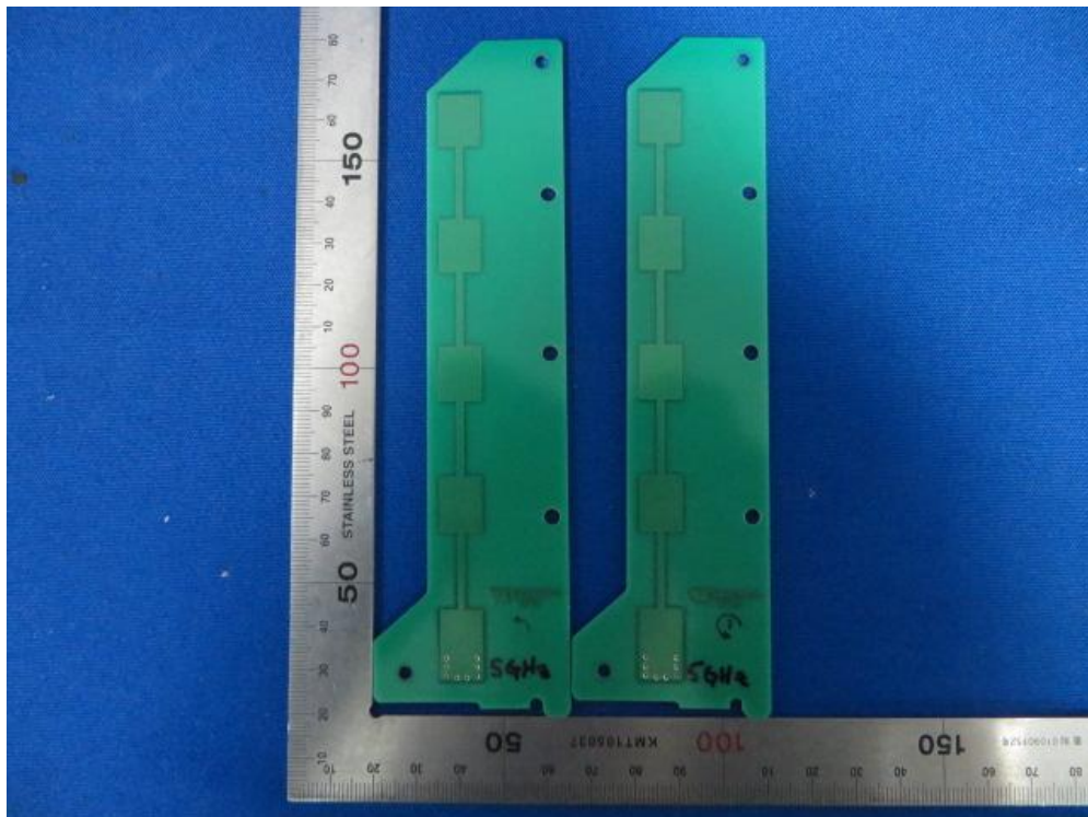
(8) EUT Photo (5GHz Antenna)
