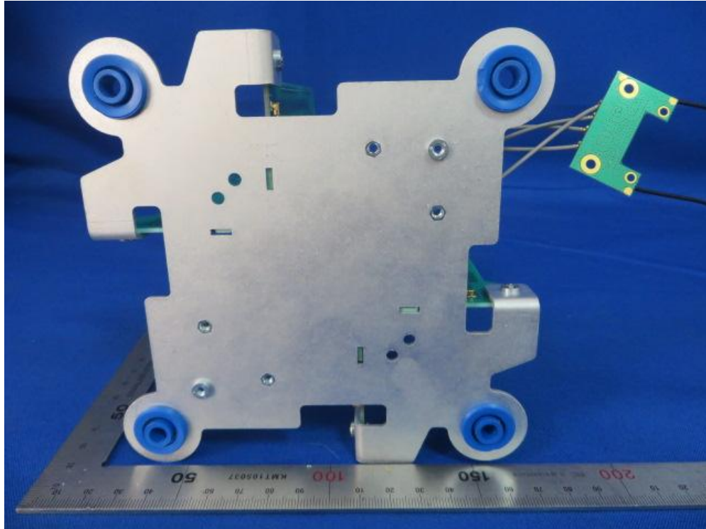
(6) EUT Photo (2.4GHz Antenna)
