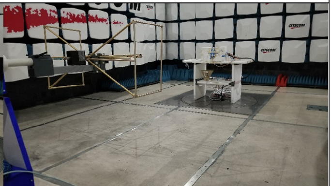
30MHz – 1GHz
